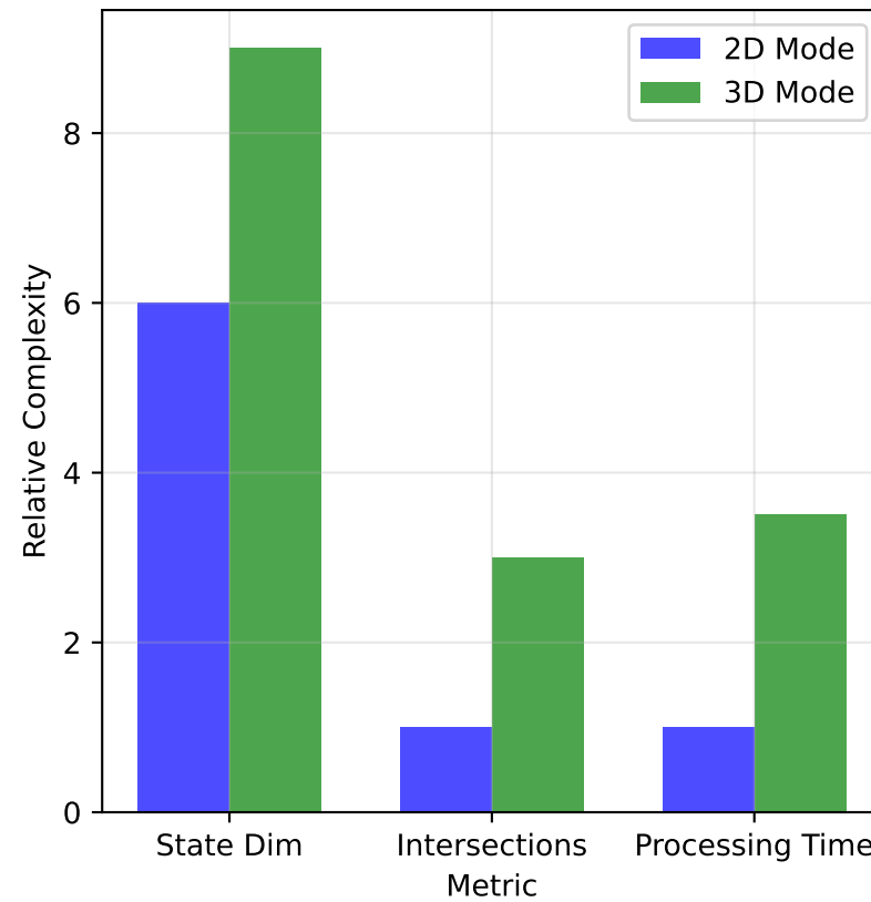
Computational Complexity
