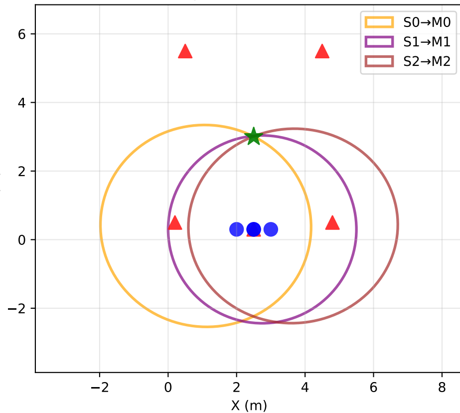
Top View (X-Y Plane) Ellipse Intersections
