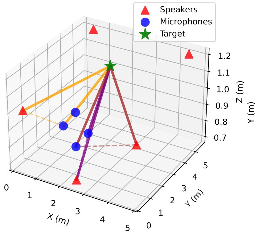
3D Ellipsoid Intersection (Acoustic Path Visualization)
