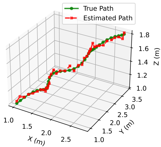
Zigzag 3D Pattern 3D Trajectory
