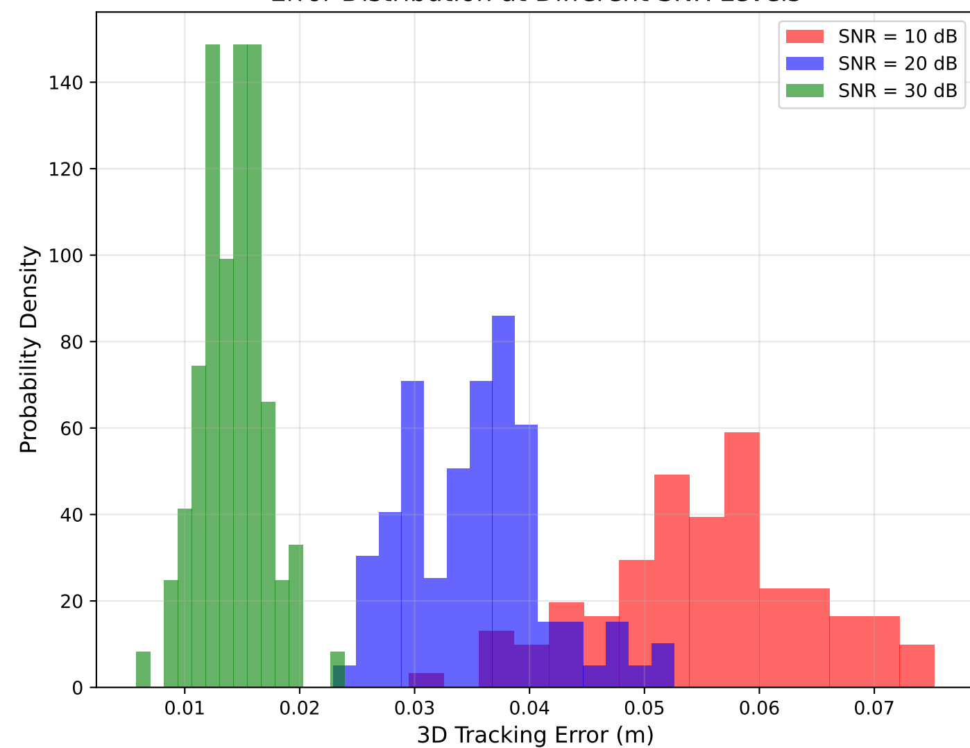
Error Distribution at Different SNR Levels
