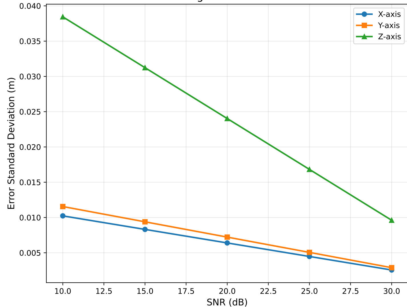
Relative Z-axis Performance vs SNR
