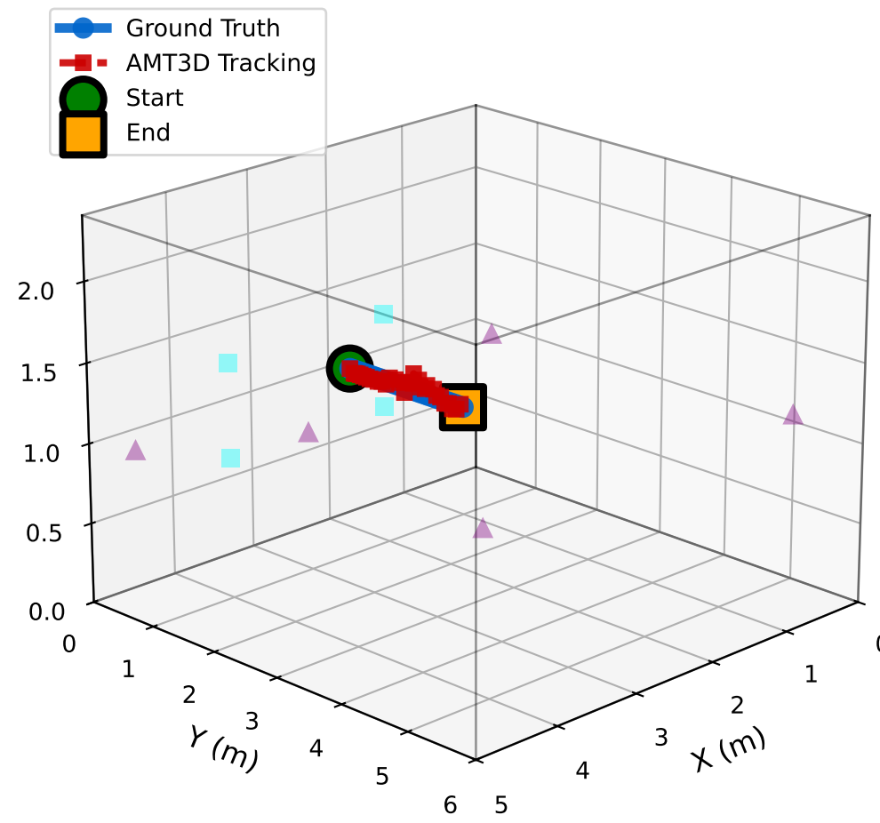
3D Tracking Performance\nMean Error: 6.5 cm
