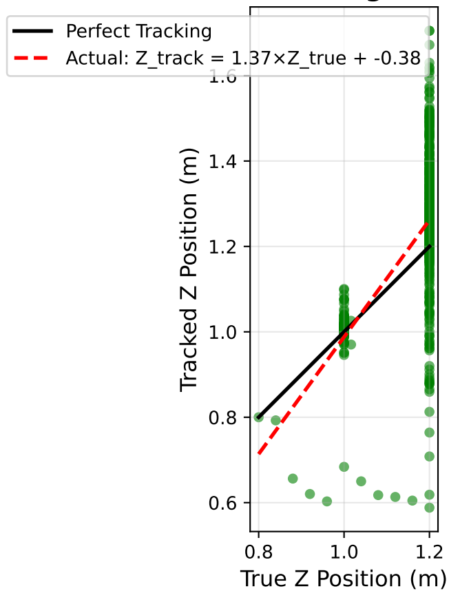
Z-axis Tracking Accuracy
