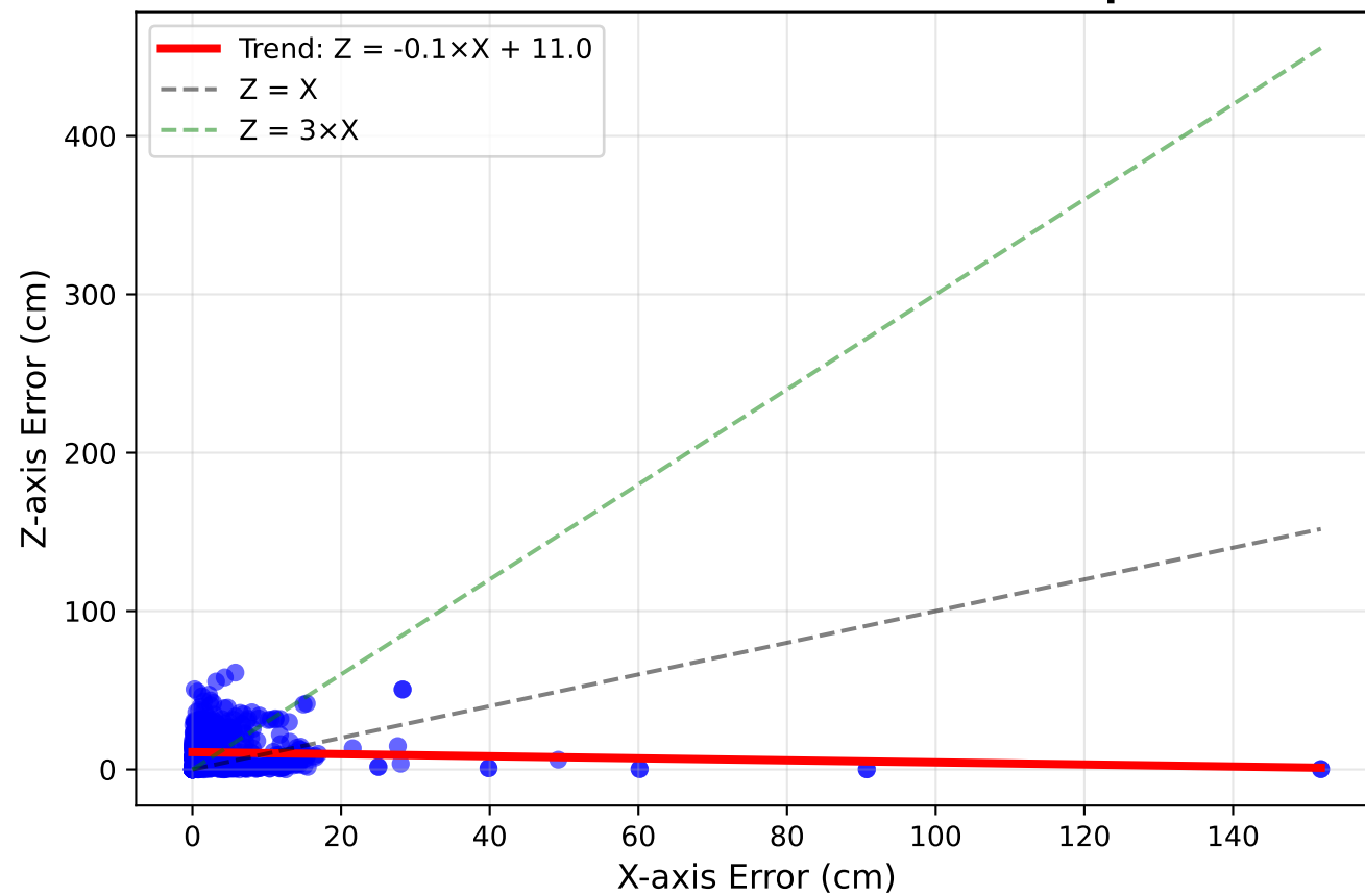
Z-axis vs X-axis Error Relationship
