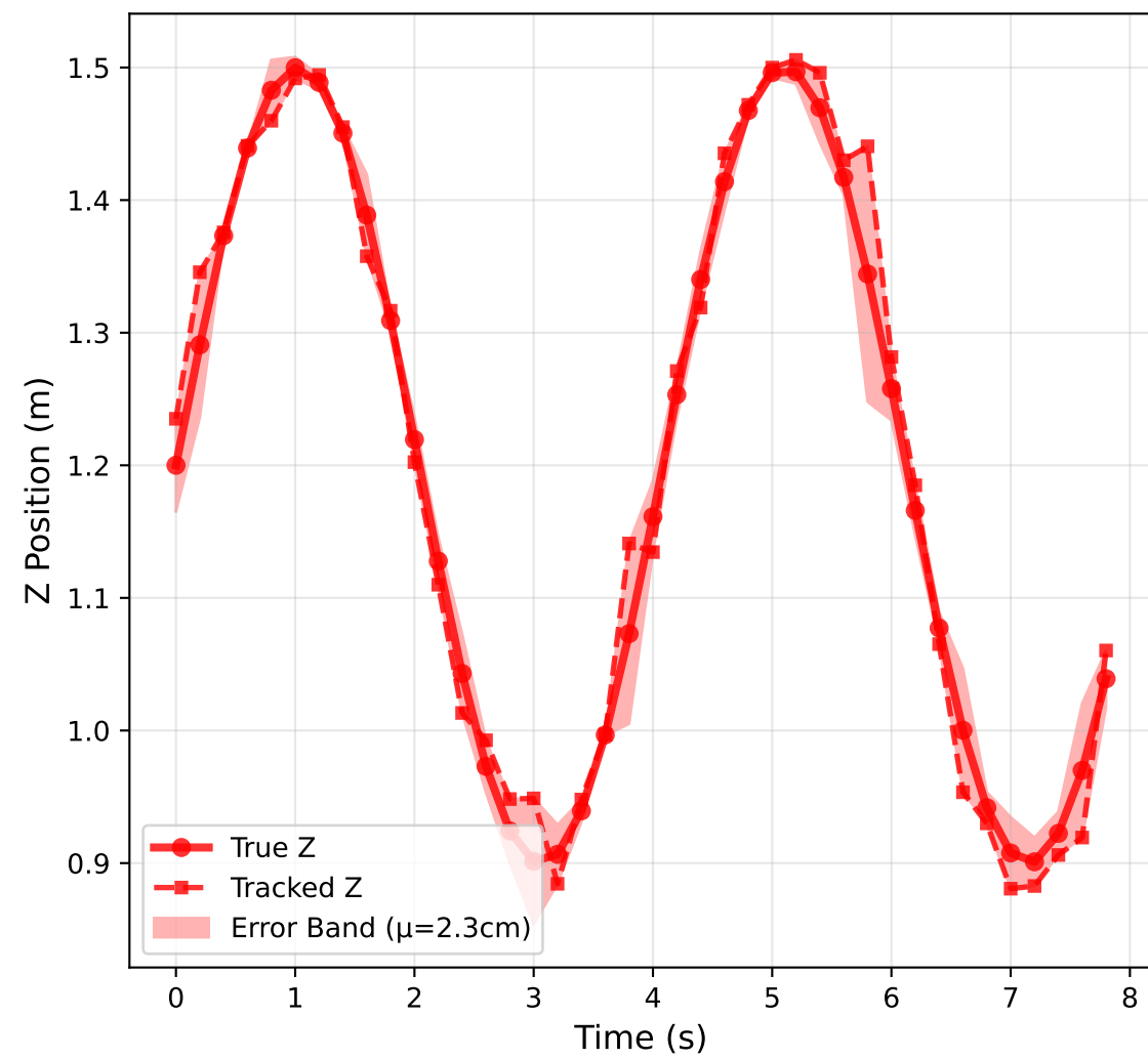
Z-axis Tracking Mean Error: 2.3cm
