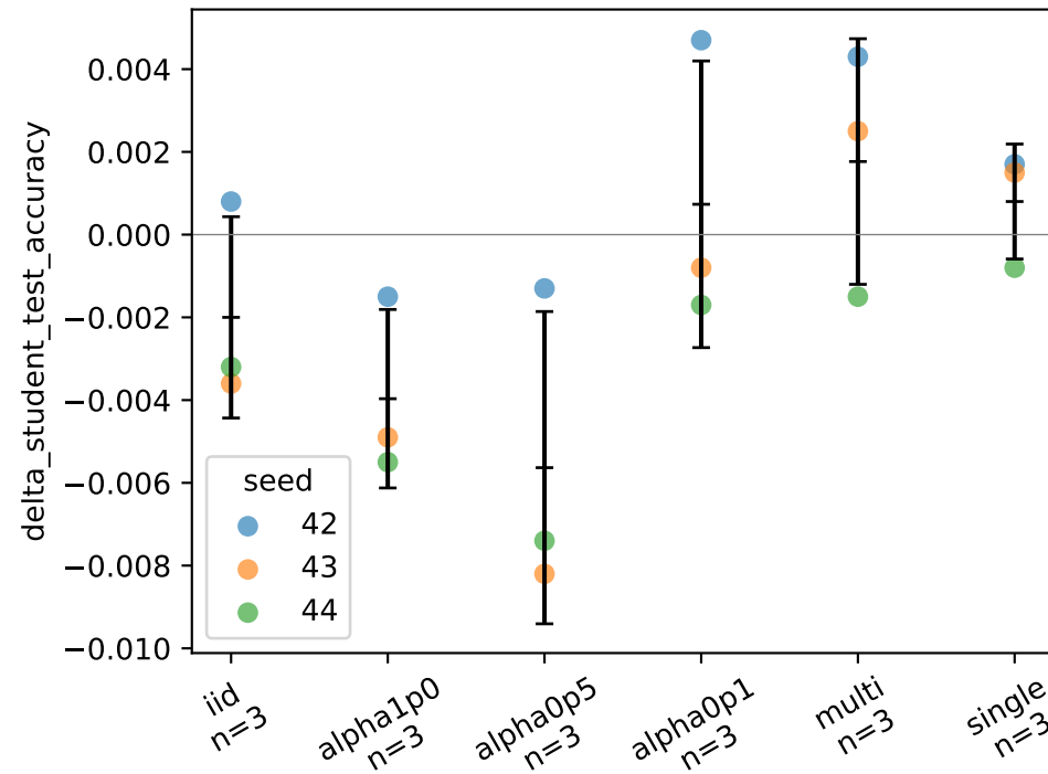
mnist · completo (3 seeds)
