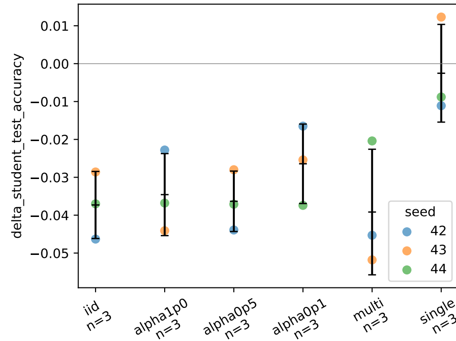
cifar · completo (3 seeds)
