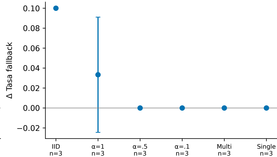
mnist · EXPERT-prob – FedDF-prob
