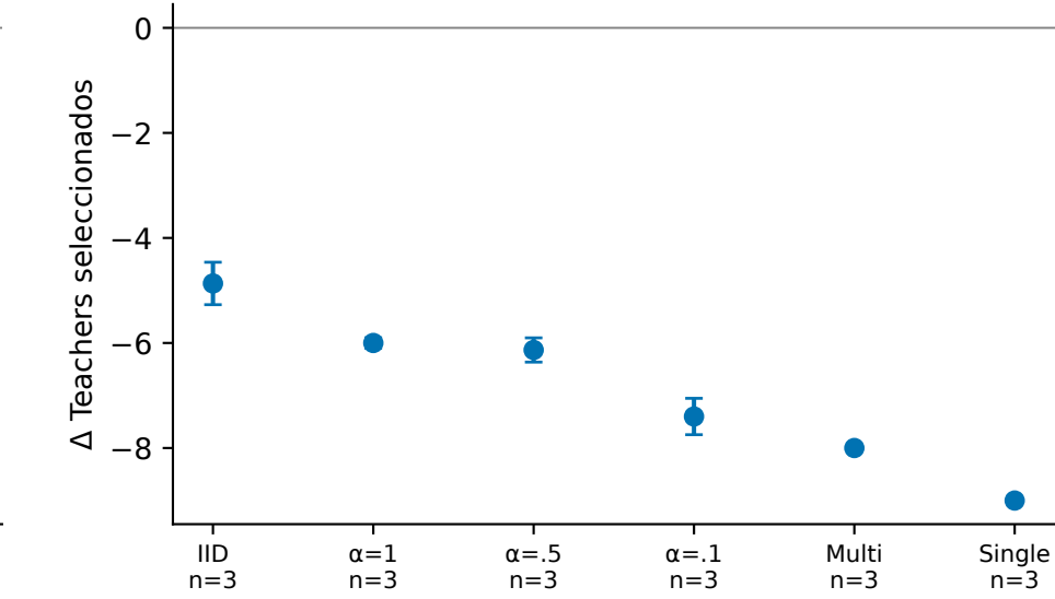
cifar · EXPERT-prob – FedDF-prob
