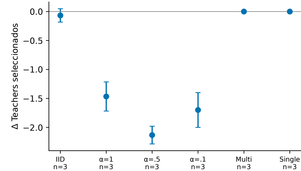
fmnist · EXPERT-prob – Presence-prob
