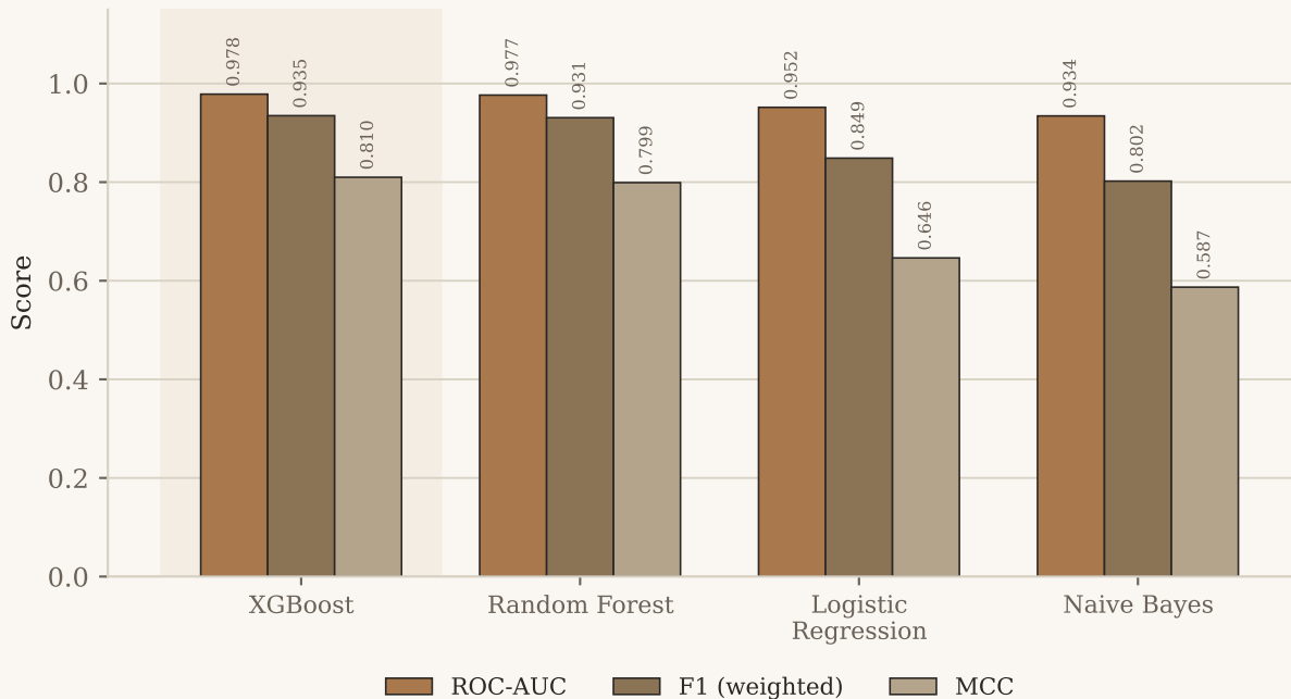
Classifier Comparison (n = 45,000 rows, 80/20 split)
