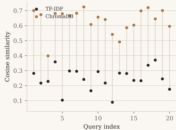
Top-1 similarity score
