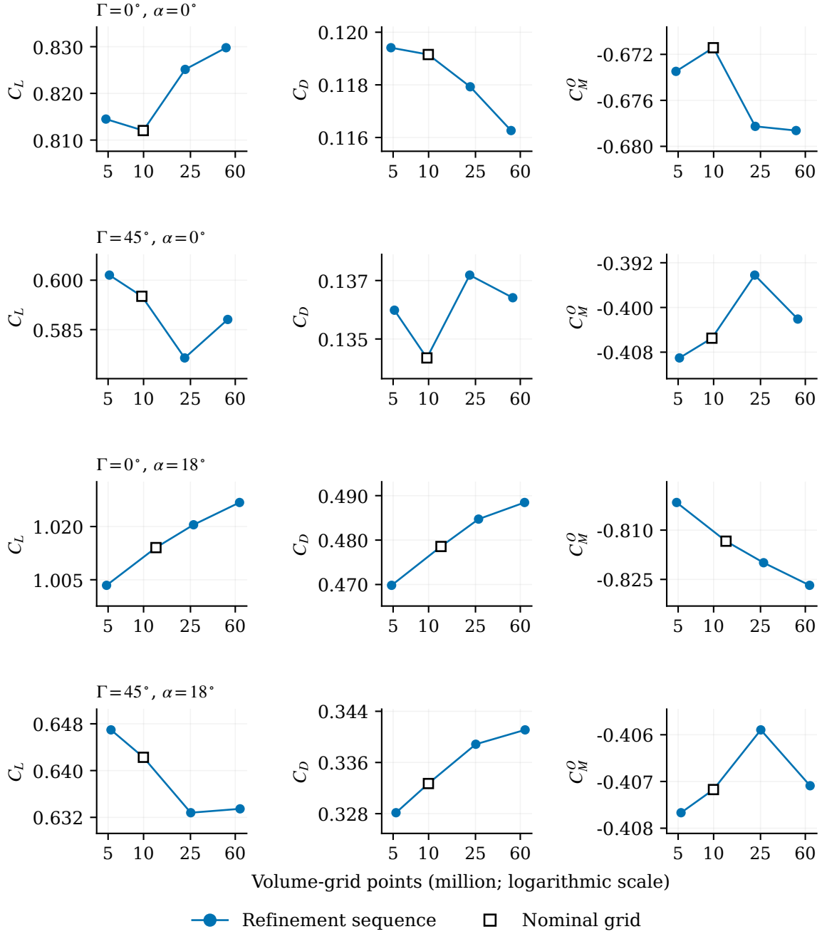
Fig. 2 Existing four-level Geom. I study at \delta = 35^\circ : rows show (\Gamma, \alpha) = (0, 0), (45, 0), (0, 18), (45, 18)^\circ ; columns show C_L, C_D, and C_M^O . The abscissa is the actual volume-grid point count on a logarithmic scale; left-to-right samples are coarse, nominal, fine, and very fine. Open squares identify nominal grids. Moments use O = (0.229, 0, 0) m and the Geom. I area/MAC. The two finest \alpha = 0^\circ moments are taken from the same terminal histories as lift and drag; the other moments use matching force reports. Volume-element counts range from 9.51 to 109.98 million. Lines connect retained refinement levels, without an asymptotic-convergence estimate.
