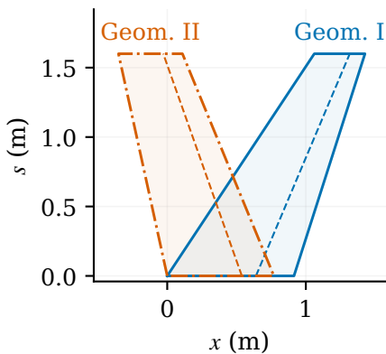
(b) Planforms; dashed hinge
