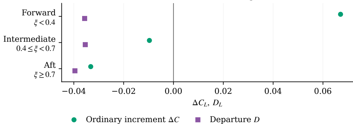
(a) Chordwise lift changes
