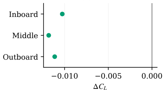
(b) Aft lift
