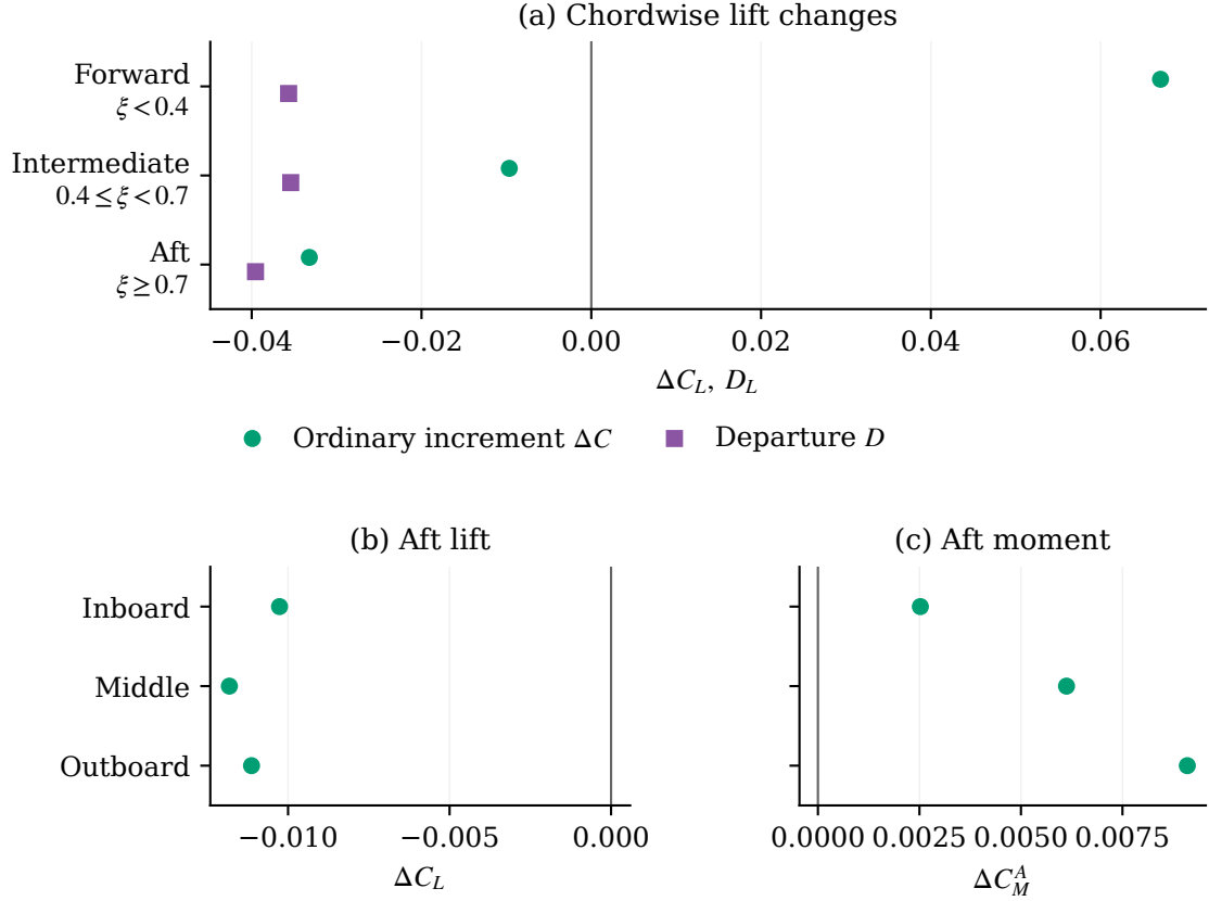
Fig. 6 Integrated geometric-region changes for I/\Gamma = 0^\circ/\delta = 20^\circ , direct 0 \rightarrow 2^\circ : (a) paired chordwise lift increments and departures; (b,c) aligned ordinary aft lift and moment increments over inboard ( \eta < 1/3 ), middle ( 1/3 \leq \eta < 2/3 ), and outboard ( \eta \geq 2/3 ) regions. Baseline: \{-6, -4, -2\}^\circ ; fitted axis: x_A = 0.642 m. Both sides and root extensions are included. Endcaps are separate in the complete total, so the displayed rows alone do not exhaust it. Points are integrated contributions, not densities or native solver marker groups.
