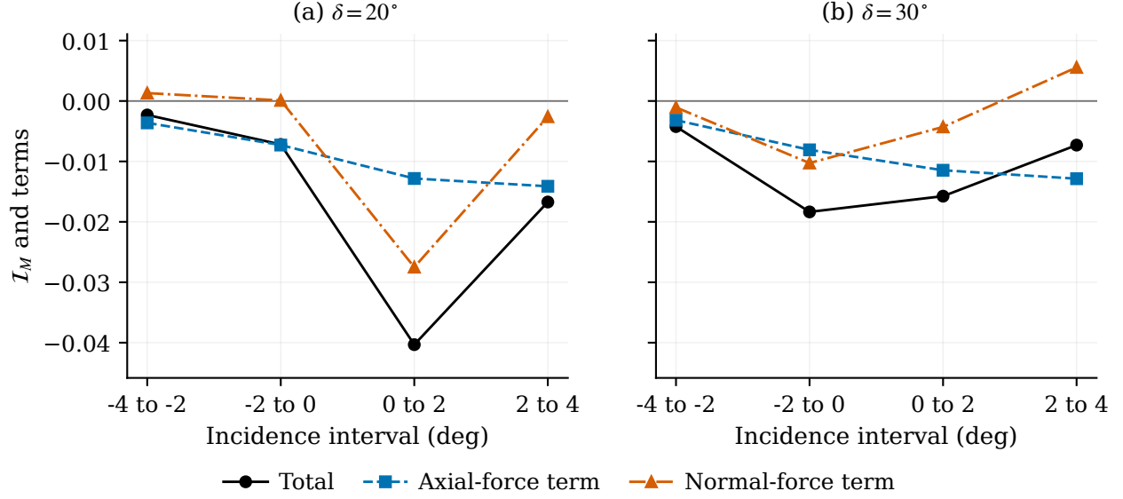
Fig. 8 Matched I dihedral contrasts of ordinary moment increments, 45^\circ minus 0^\circ , at \delta = 20^\circ (a) and 30^\circ (b). Moment uses common numerical axis A_I = (0.642, 0, 0) m. The axial- and normal-force series are interval contrasts of the two normalized integrated terms in Eq. 5, whose sum is I_M in Eq. 6. Each marker represents its labeled 2^\circ interval; lines guide the eye between interval summaries. Direct zero parents are used, without baseline subtraction.
