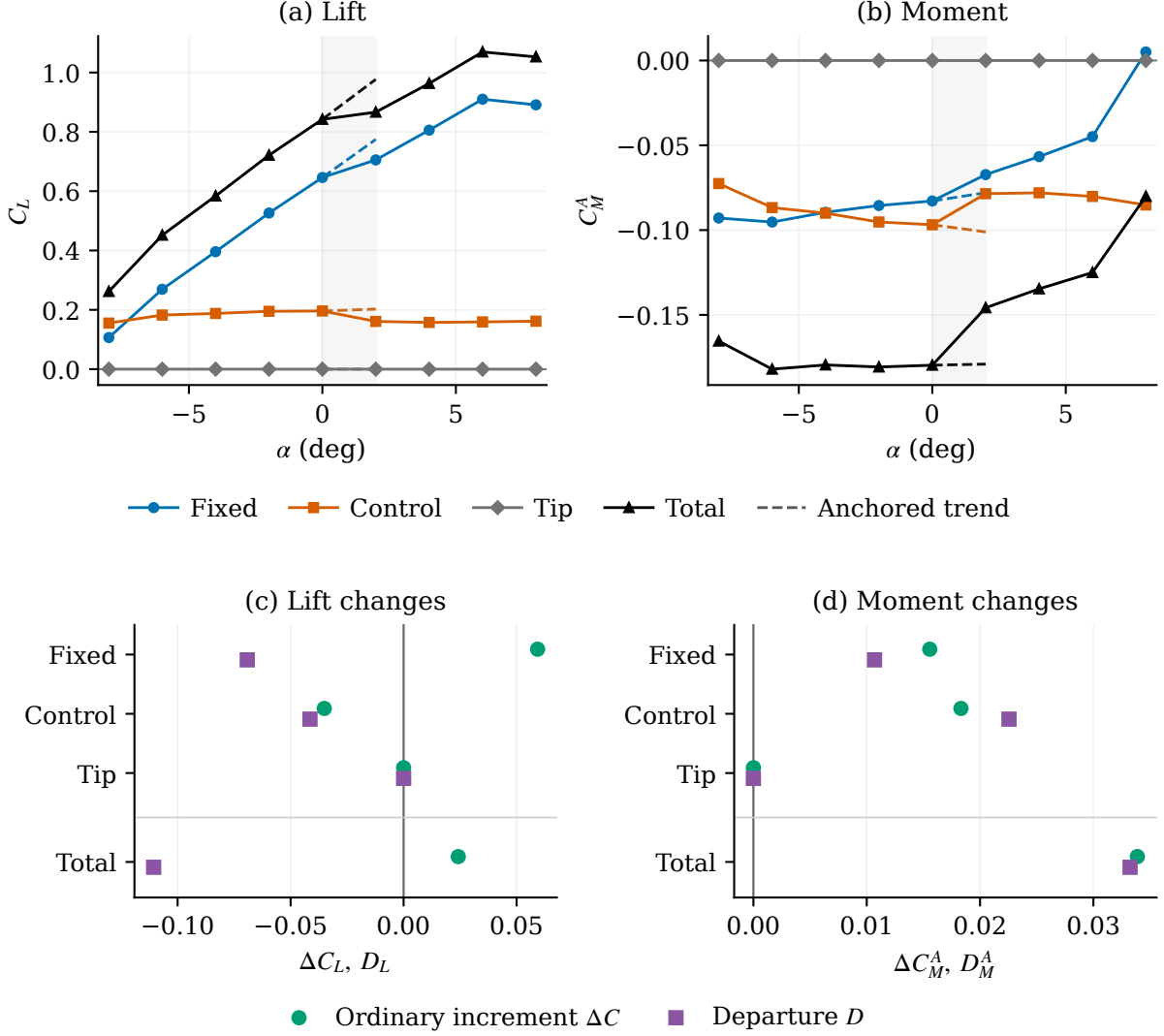
Fig. 4 I/\Gamma = 0^\circ/\delta = 20^\circ : component coefficients (a,b) and signed ordinary-increment/departure pairs (c,d). Dashed segments continue the stored preceding slopes from the actual direct-zero coefficients, so their endpoint gaps equal the departures in Eq. 3. Slopes use \{-6, -4, -2\}^\circ ; shading marks direct 0 \rightarrow 2^\circ . All components, including tip, use global area/MAC and fitted axis x_A = 0.642 m. Total is separated from the component rows; points have no uncertainty-bar interpretation.
