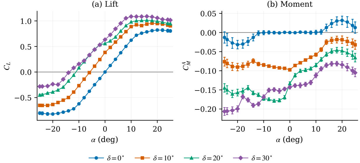
Fig. 2 LE1 WT response of Geom. I, \Gamma = 0^\circ , for \delta = 0, 10, 20, 30^\circ . Moment C_M^A uses the experimental zero-deflection fitted center, held fixed across deflection. Bars are the paired supplied propagated magnitudes, without an assigned common coverage factor.
