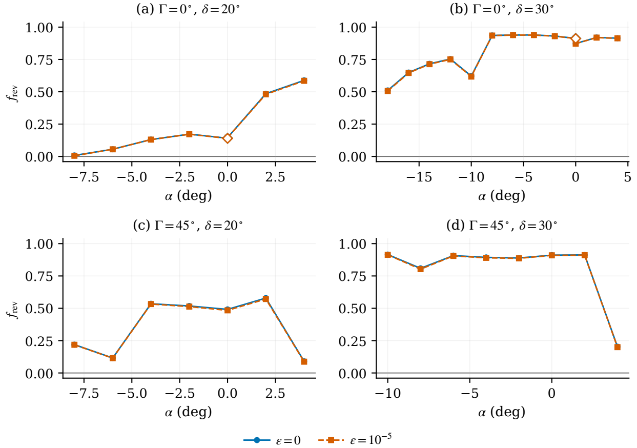
Fig. 7 Upper geometric-aft chordwise reversal fractions for I at both dihedral settings and \delta = 20, 30^\circ . Actual triangle area supplies the denominator. Circles/solid: \epsilon = 0 ; squares/dashed: \epsilon = 10^{-5} . Open diamonds identify reflected zero-incidence parents. All selected samples, including the nonmonotonic inclined 4^\circ states, are shown. The indicator measures reversed chordwise wall shear over the specified region.
