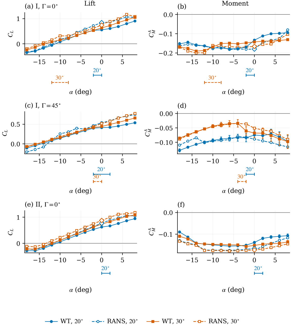
Fig. 3 WT-RANS comparison of lift and moment for I/\Gamma = 0^\circ (a,b), I/\Gamma = 45^\circ (c,d), and II/\Gamma = 0^\circ (e,f). Filled/solid: LE1 WT; open/dashed: RANS. Circles and squares distinguish \delta = 20^\circ and 30^\circ . Separate strips show selected WT intervals, subject to the uncertainty discussion. Open diamonds identify reflected zero-incidence parents. Moment uses each dataset's zero-deflection fitted center; direct and reflected branches remain separate.
