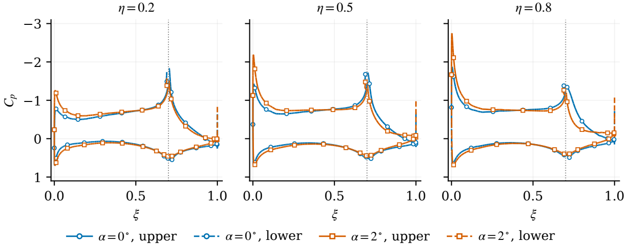
Fig. 5 Pressure sections for I/\Gamma = 0^\circ/\delta = 20^\circ at direct \alpha = 0, 2^\circ and undeformed \eta = s/b = 0.2, 0.5, 0.8 . Circles/squares distinguish incidence; solid/dashed lines distinguish upper/lower sides. Segments preserve native main-panel contour connectivity, excluding junction, tip, and blunt-edge faces. The vertical dotted line marks the 70%-chord hinge. \xi is the local chord fraction obtained by undoing the hinge rotation.
