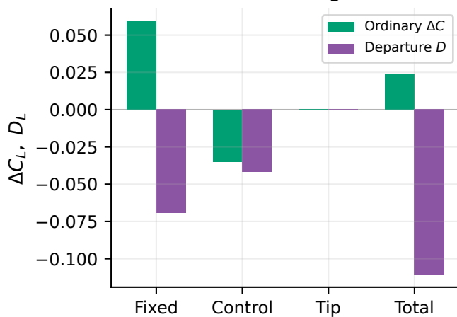
(c) Lift changes
