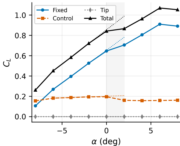
(c) Lift changes
