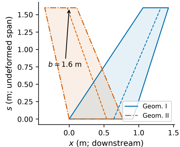
(b) Planforms; dashed 70% hinge
