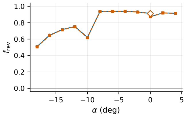
(b) I, \Gamma = 0^\circ, \delta = 30^\circ
