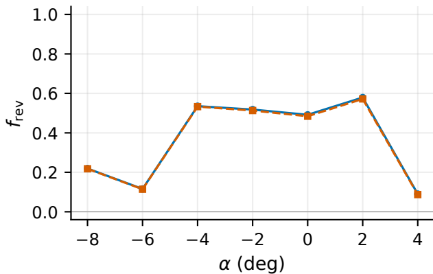
(c) I, \Gamma = 45^\circ, \delta = 20^\circ
