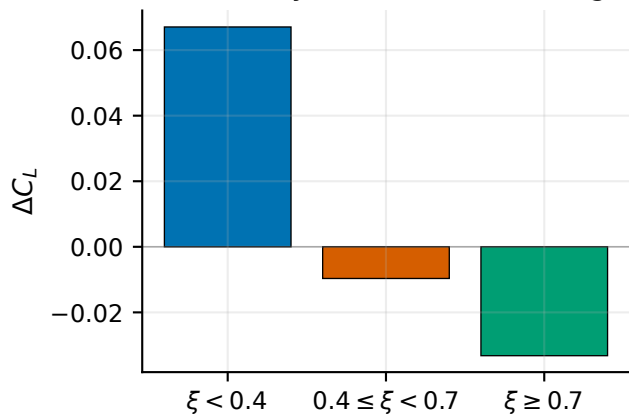
(a) Ordinary chordwise lift changes
