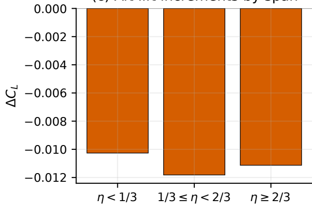
(c) Aft lift increments by span
