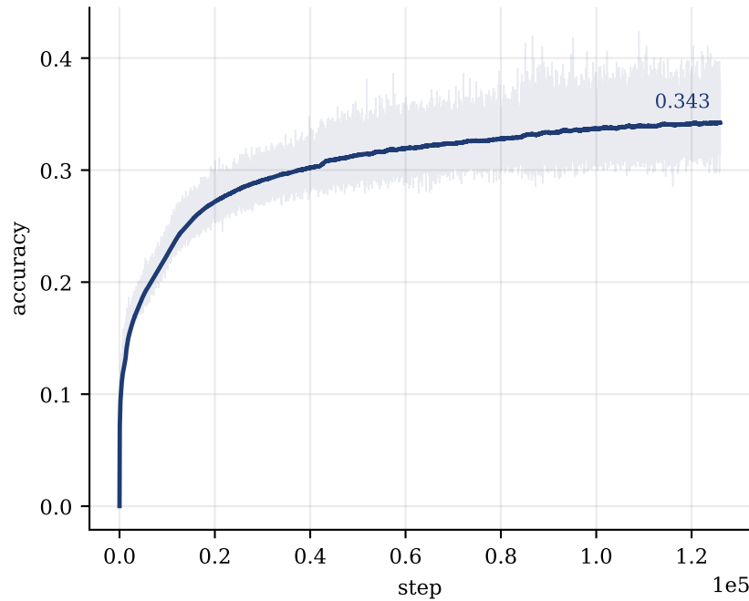
next-token prediction accuracy
