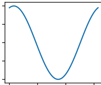
Phase = 2\pi/5
