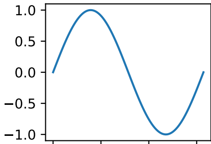
Phase = 0\pi/5
