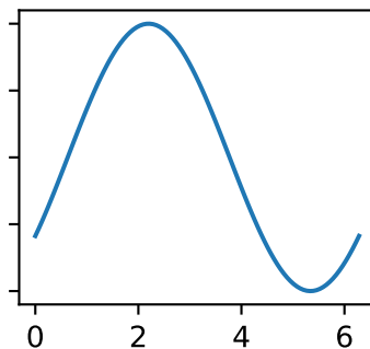
Phase = 9\pi/5
