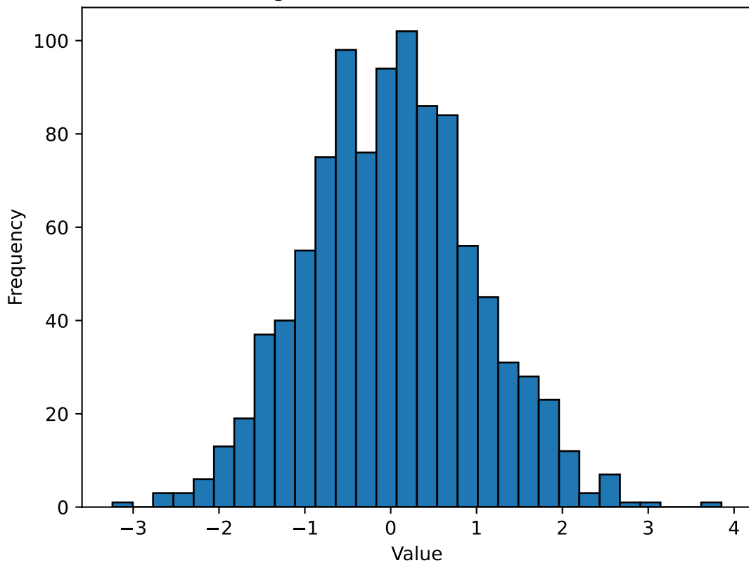
Histogram of Standard Normal Data
