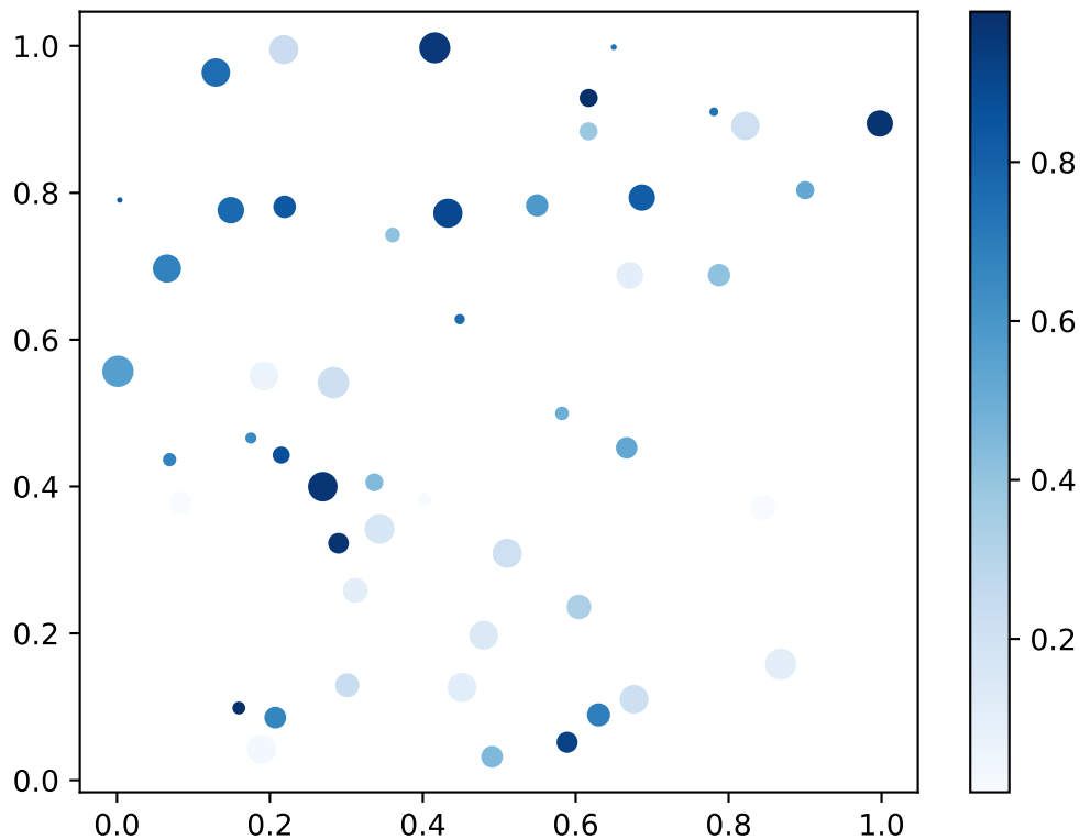
Random Scatter Plot
