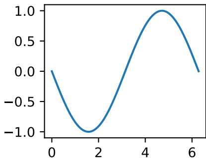
Phase = 5\pi/5
