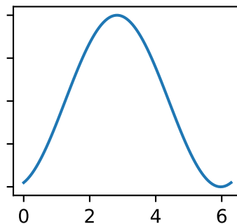
Phase = 8\pi/5
