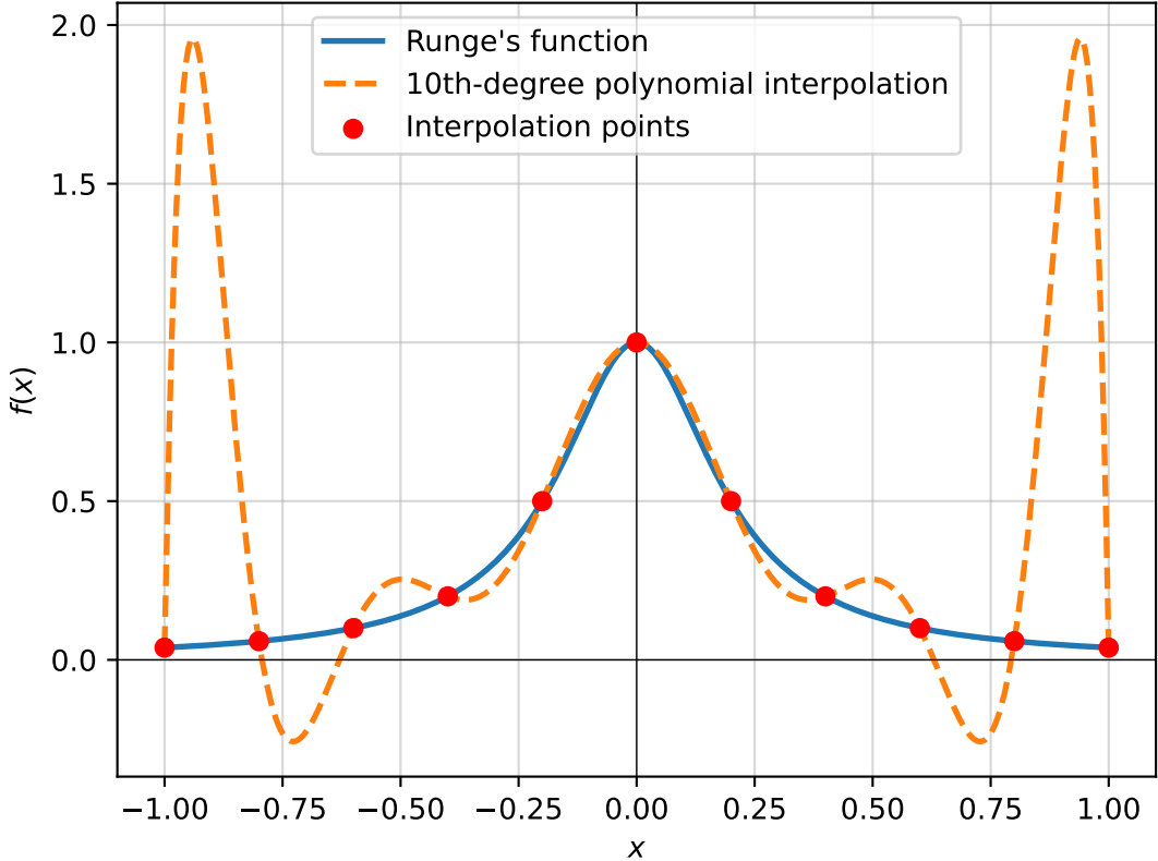
Runge's Phenomenon: Oscillations in High-Degree Polynomial Interpolation
