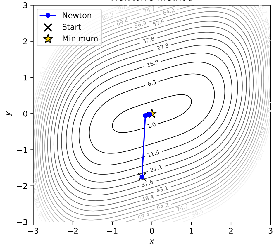
Newton's method
