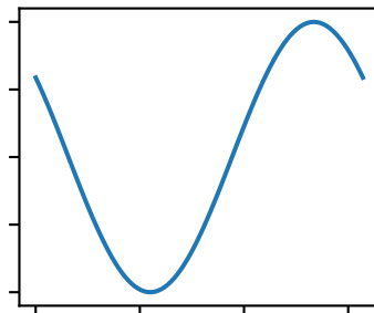
Phase = 4\pi/5
