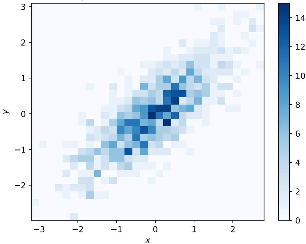
2D Histogram of Correlated Normal Variables
