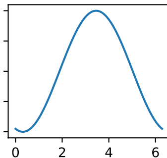
Phase = 7\pi/5
