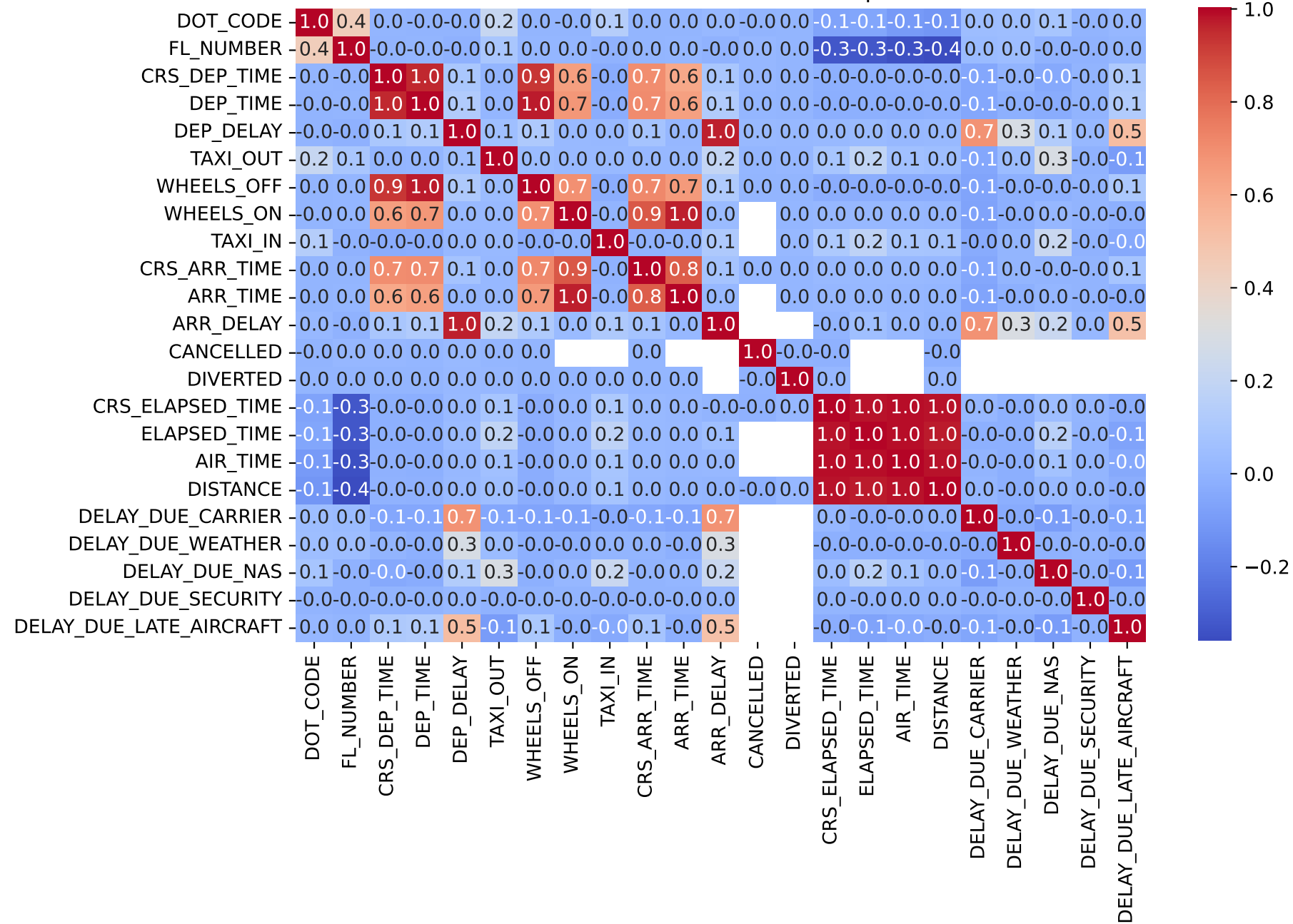
Correlation Matrix Heatmap
