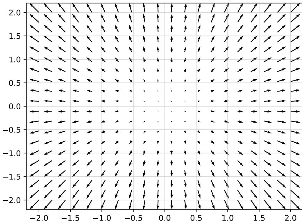
Gradient Field of f(x, y) = x^2 + y^2
