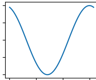
Phase = 3\pi/5
