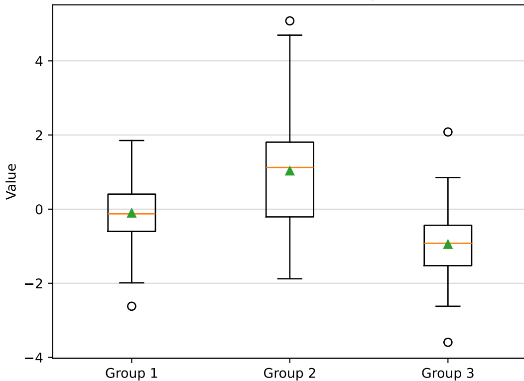
Box Plot of Three Groups
