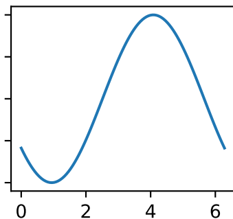
Phase = 6\pi/5
