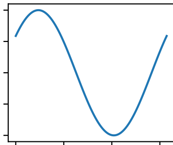
Phase = 1\pi/5
