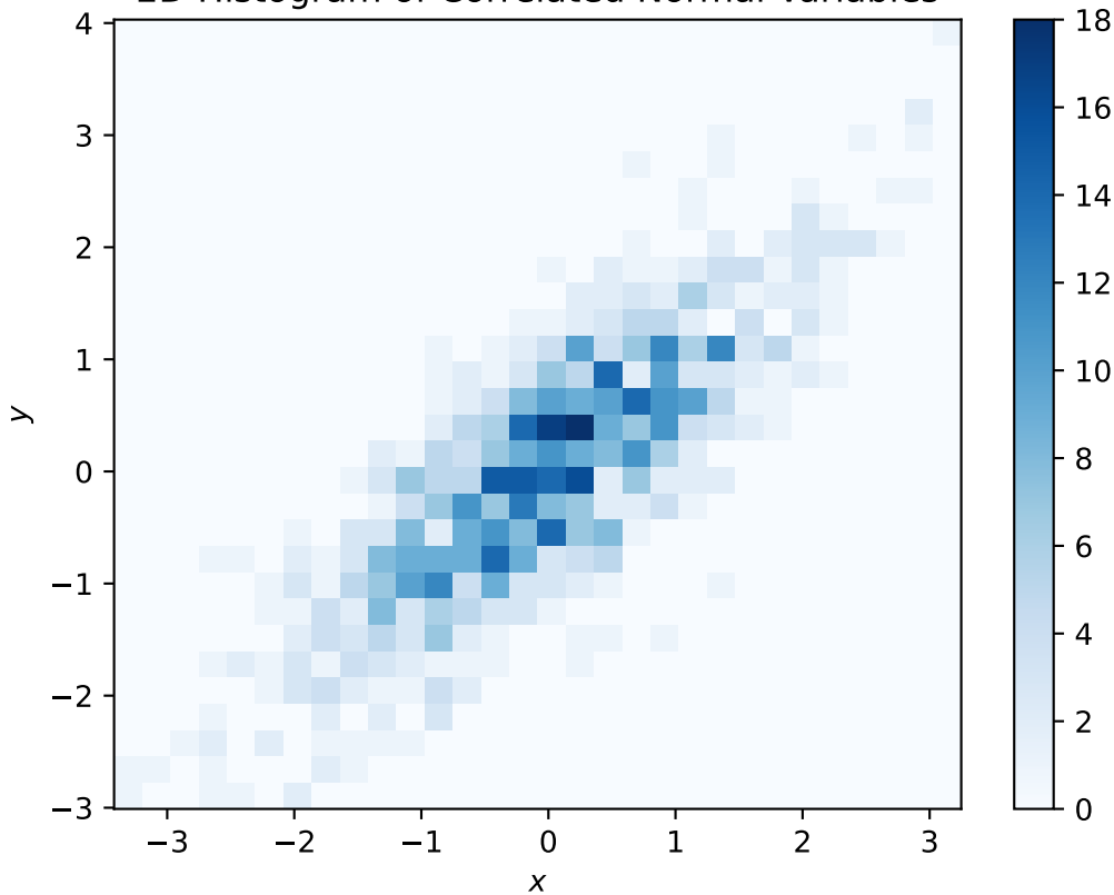
2D Histogram of Correlated Normal Variables
