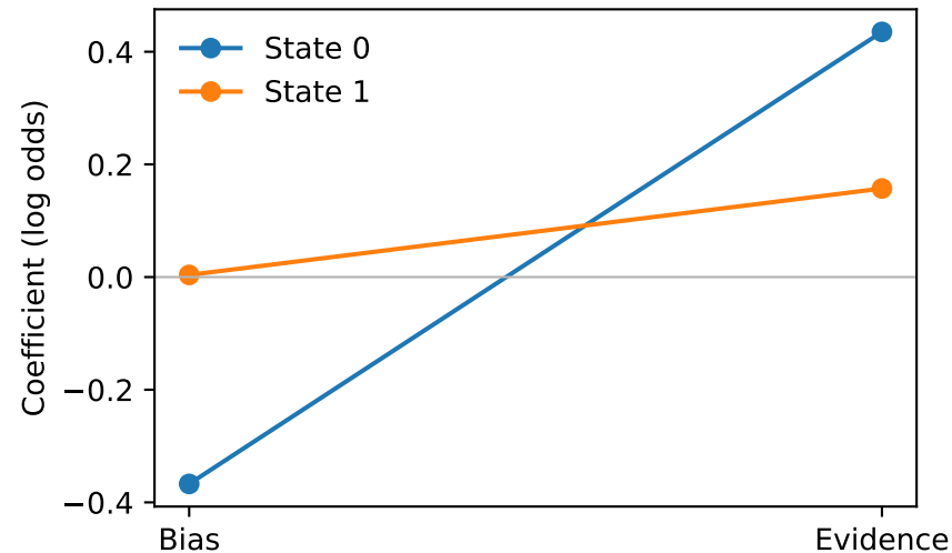
Choice-GLM identity
