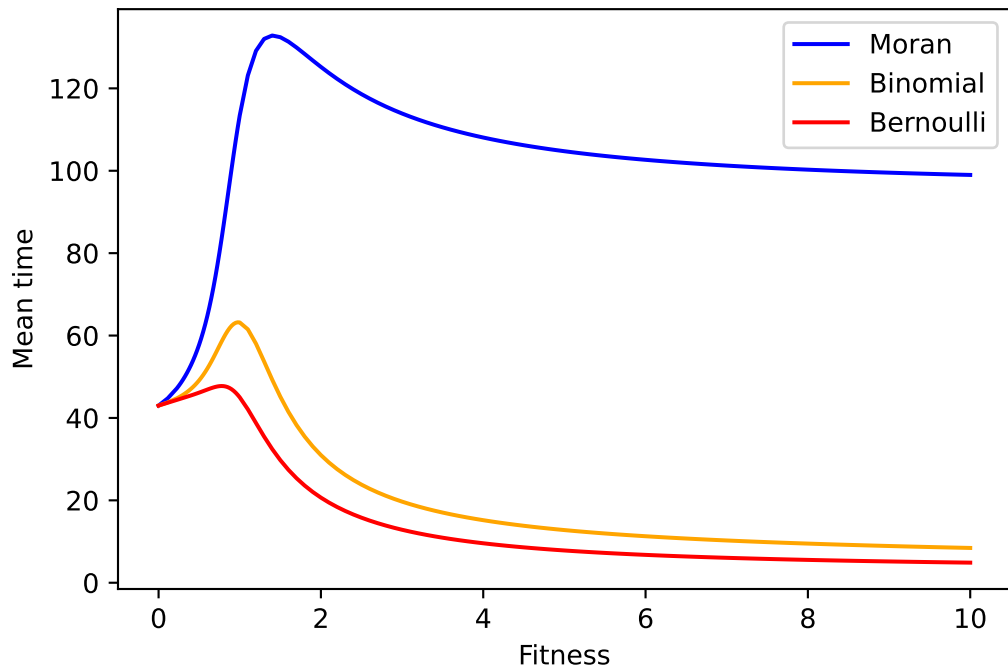
Time to absorption in K_{1,7} for p_c
