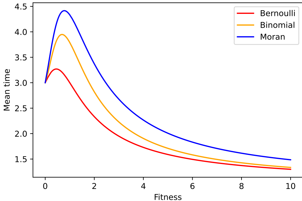
Time to extinction in K_4 for p_c
