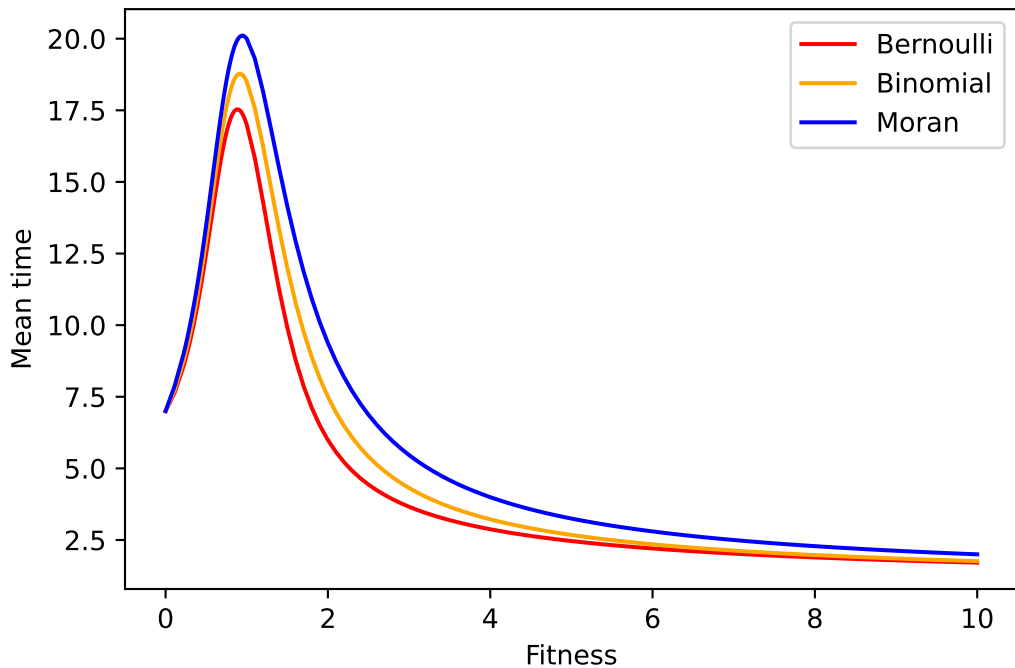
Time to extinction in C_8 for p_c
