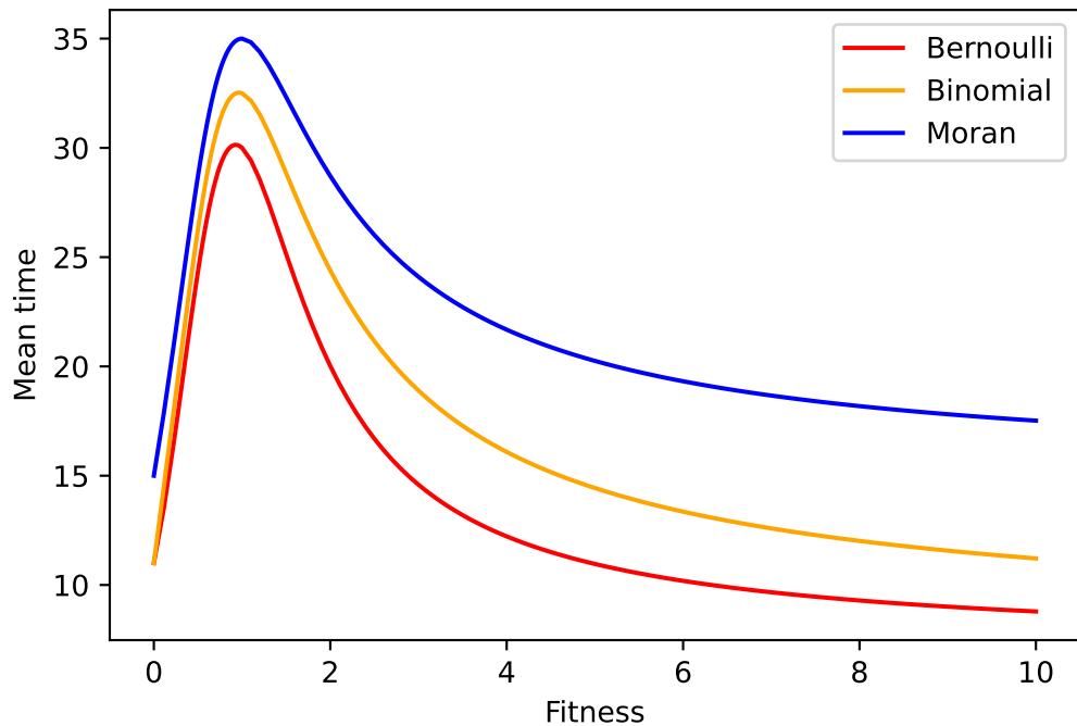
Time to fixation in C_6 for p_c
