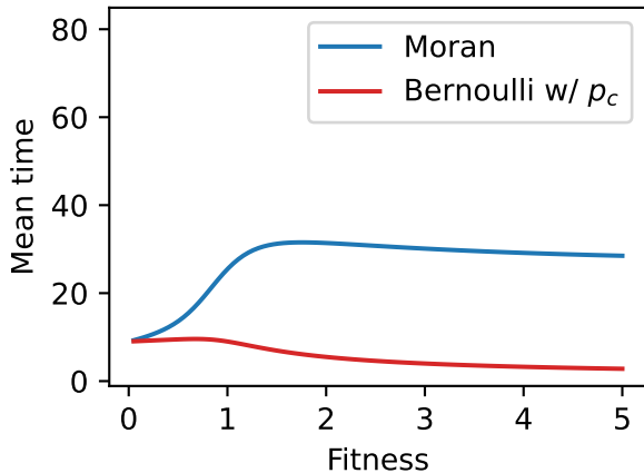
Absorption time on K_{10}
