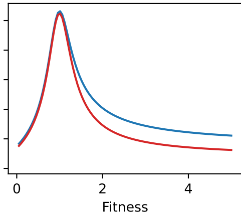
Fixation time on C_{20}
