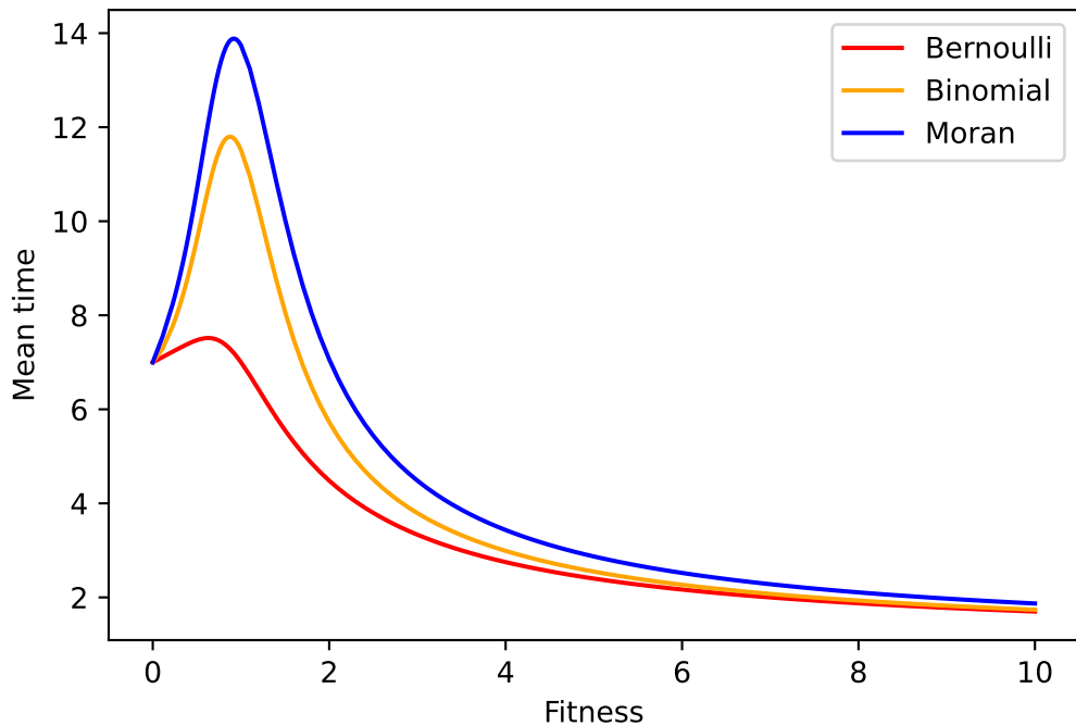
Time to extinction in K_8 for p_c
