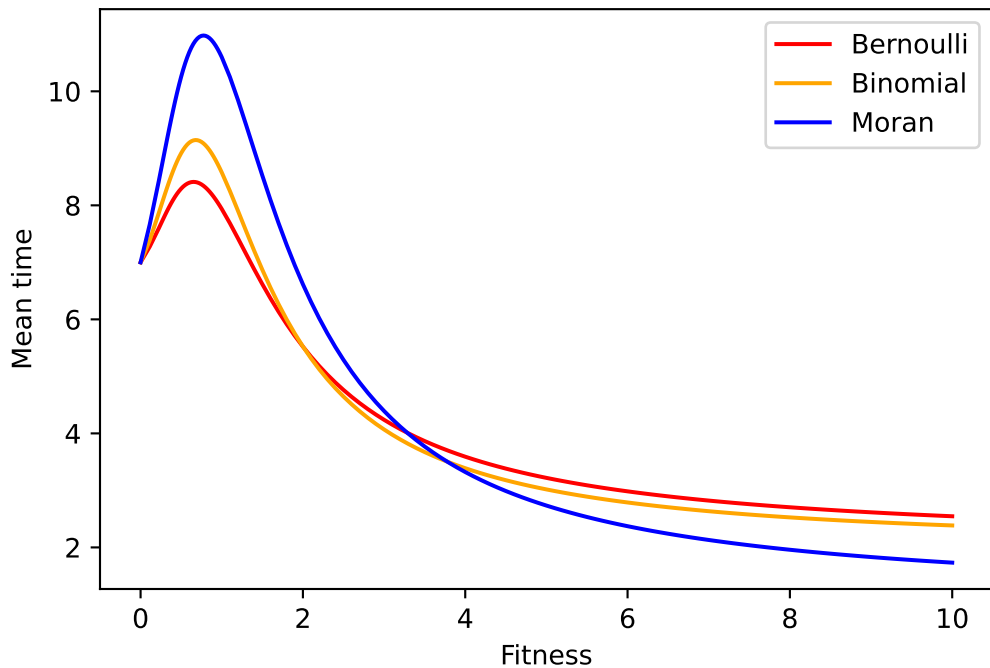
Time to extinction in K_{1,3} for p_c
