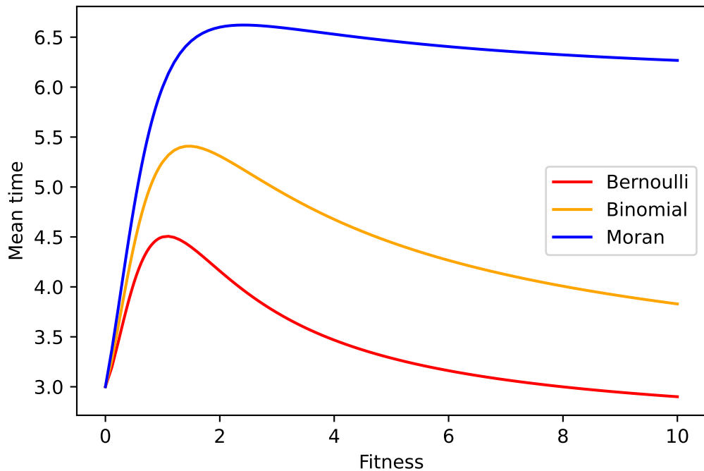
Time to absorption in C_4 for p_c
