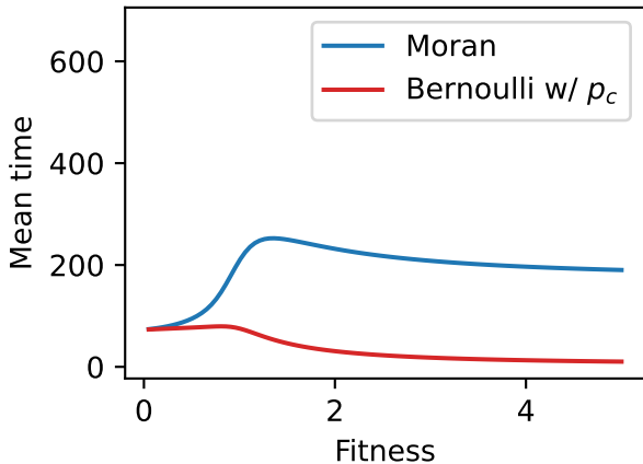
Absorption time on K_{1,9}
