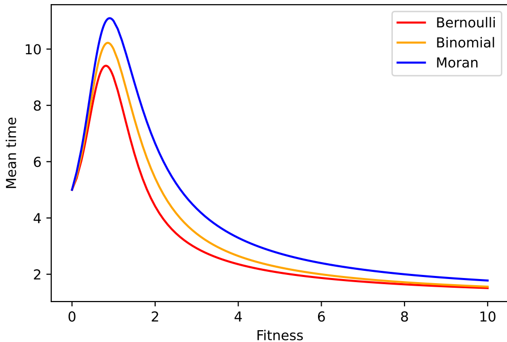
Time to extinction in C_6 for p_c
