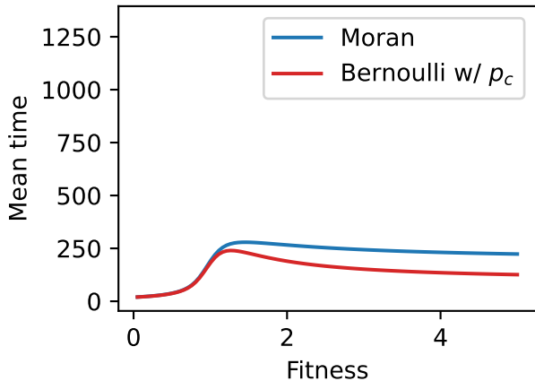
Absorption time on C_{20}
