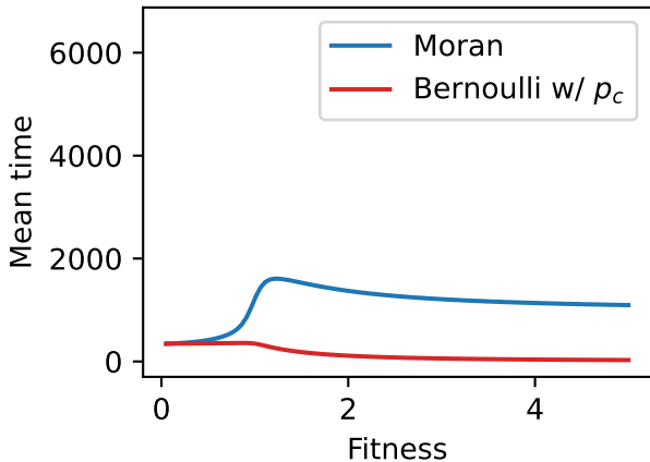
Absorption time on K_{1,19}
