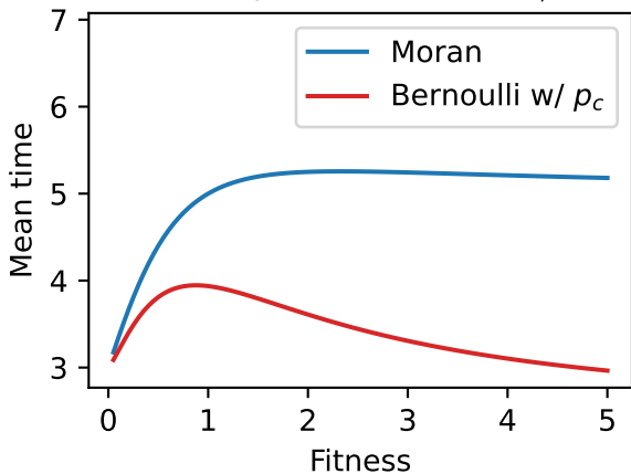
Absorption time on K_{1,2}
