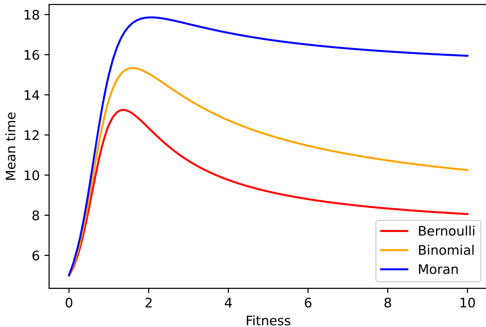
Time to absorption in C_6 for p_c
