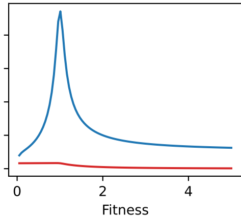
Fixation time on K_{1,29}
