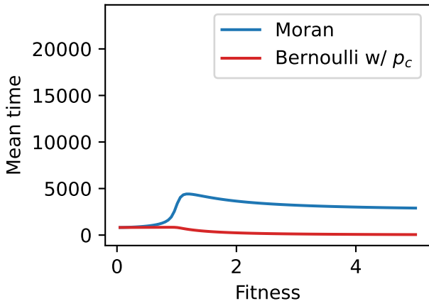
Absorption time on K_{1,29}
