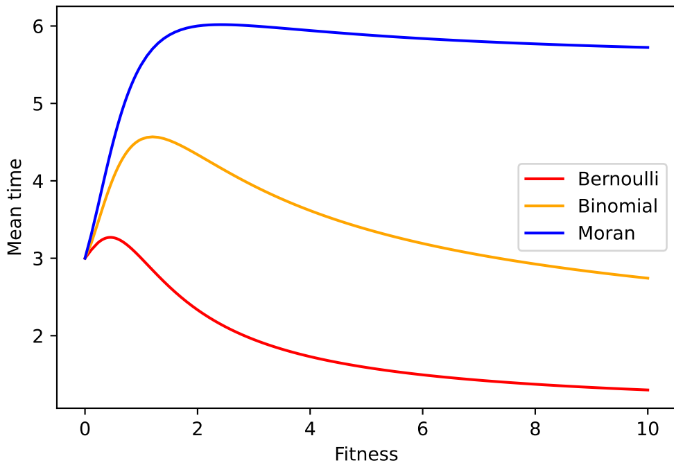
Time to absorption in K_4 for p_c
