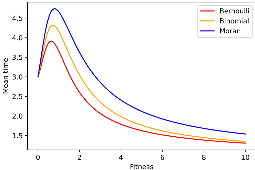
Time to extinction in C_4 for p_c
