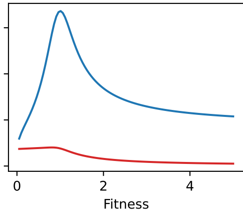
Fixation time on K_{1,9}
