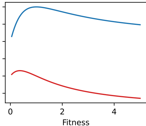
Fixation time on K_3
