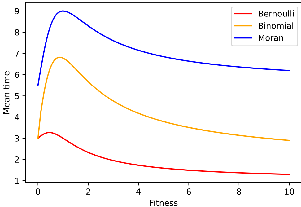
Time to fixation in K_4 for p_c
