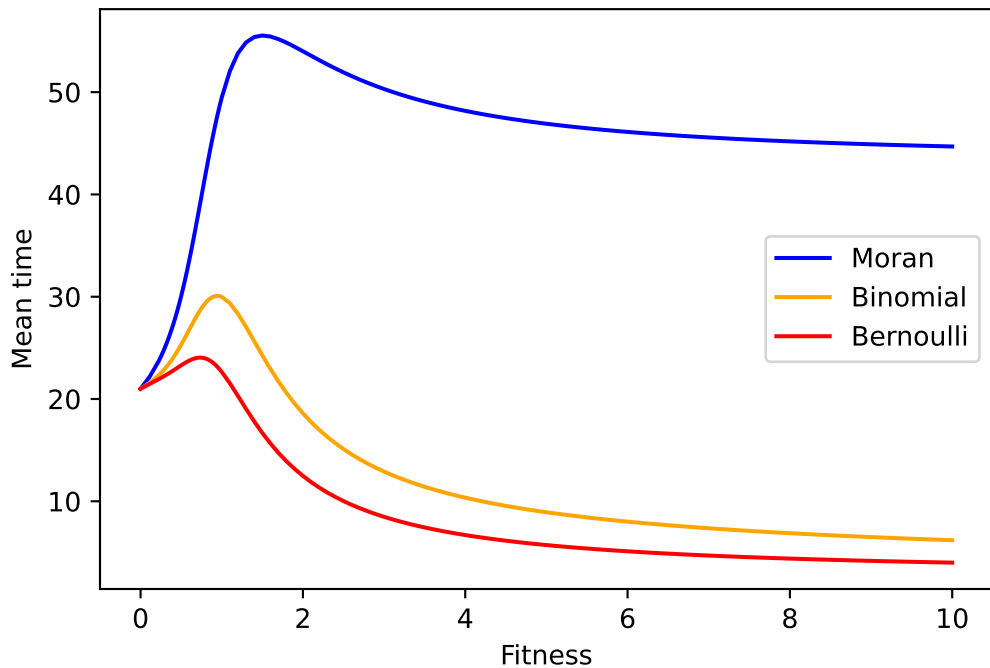
Time to absorption in K_{1,5} for p_c
