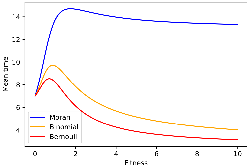
Time to absorption in K_{1,3} for p_c
