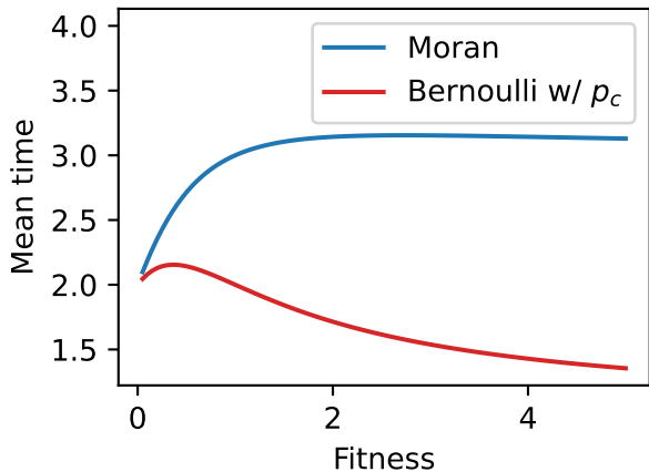
Absorption time on K_3
