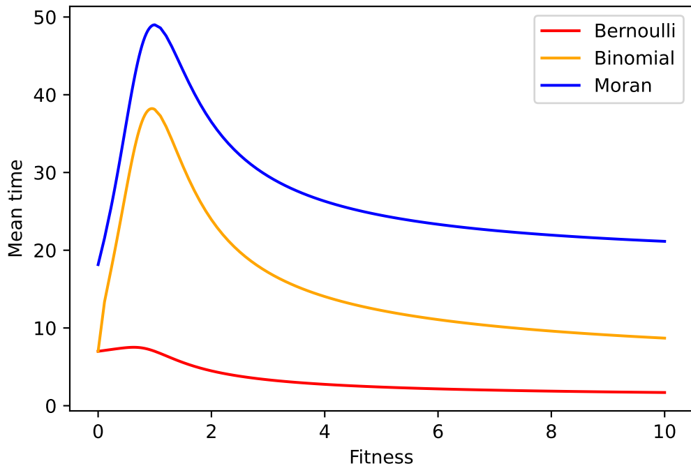
Time to fixation in K_8 for p_c
