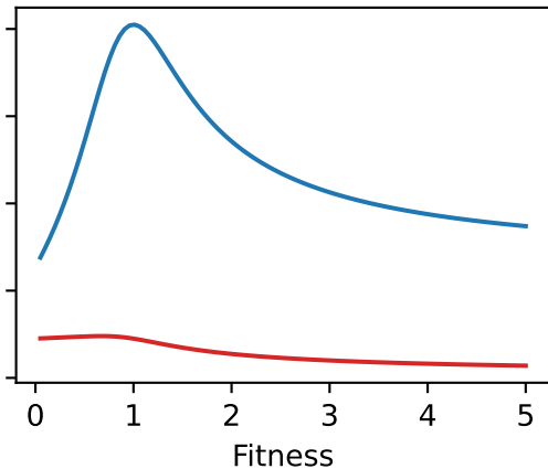
Fixation time on K_{10}
