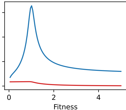
Fixation time on K_{1,19}
