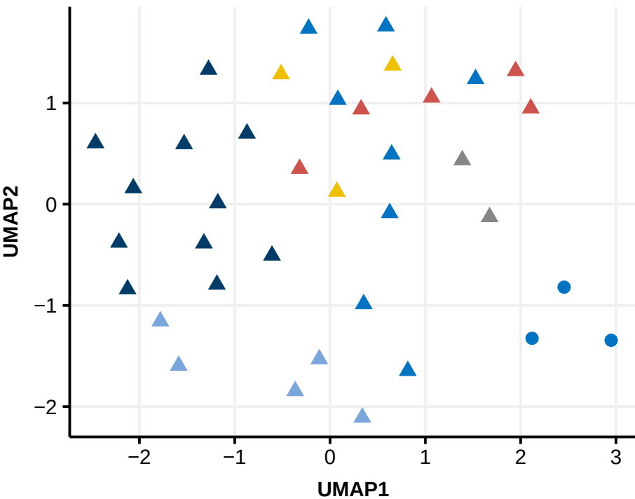
UMAP: Condition
