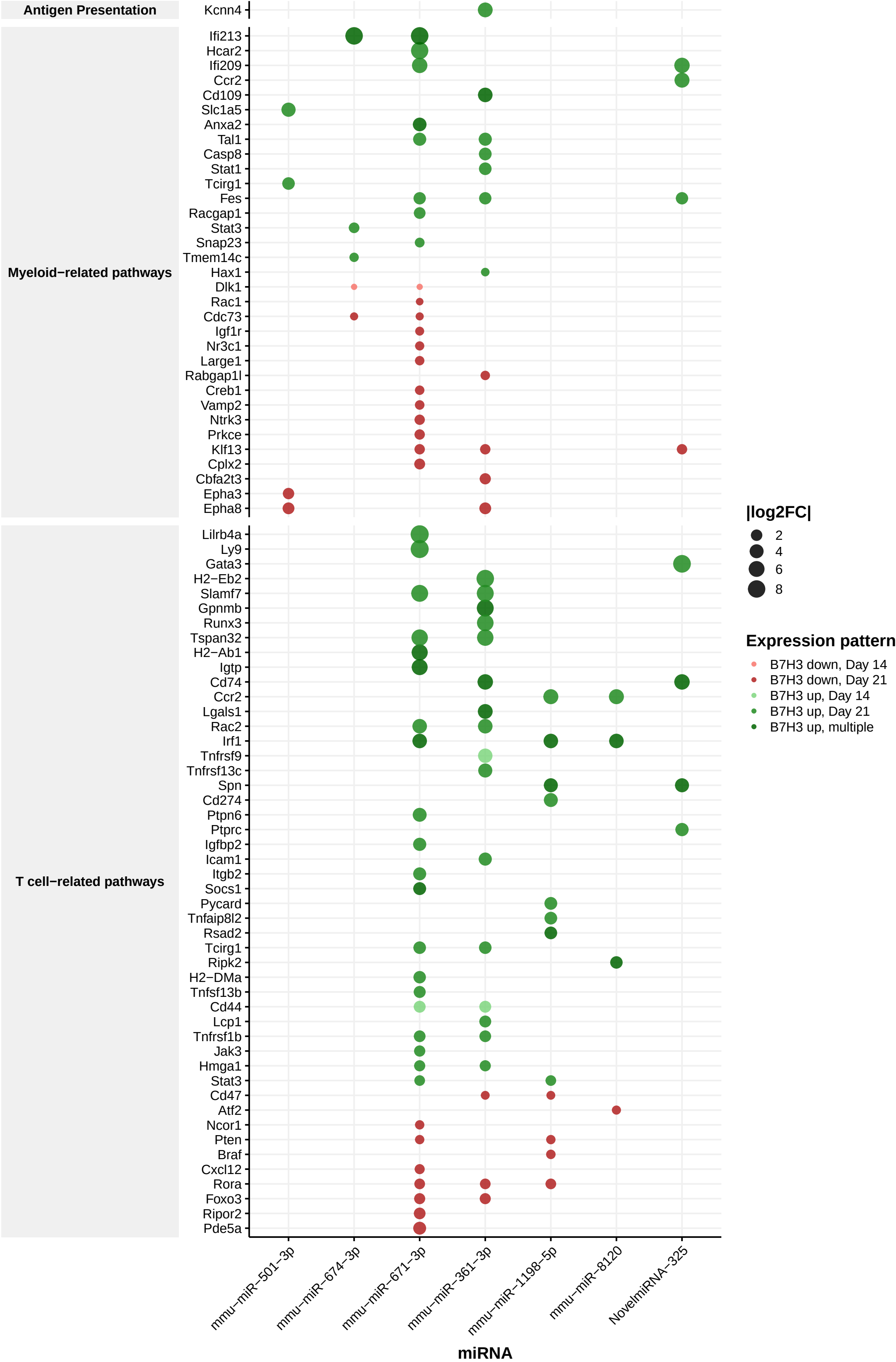
miRNA-Immune Target Interactions (Full - cluster1)
