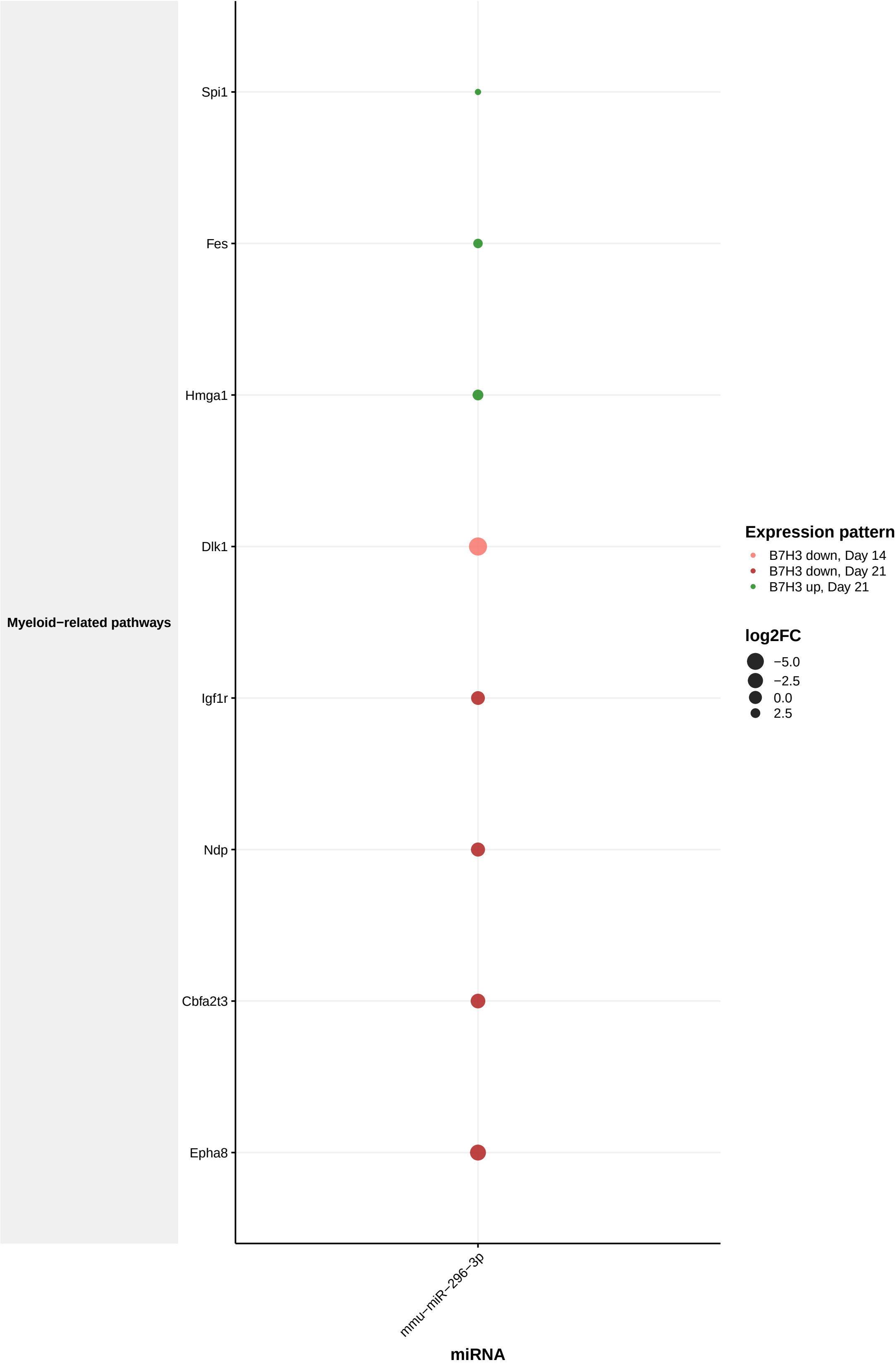
miRNA-Immune Target Interactions (Full - cluster4)
