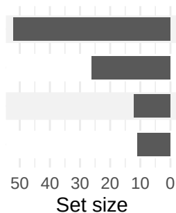
Set sizes (Down)
