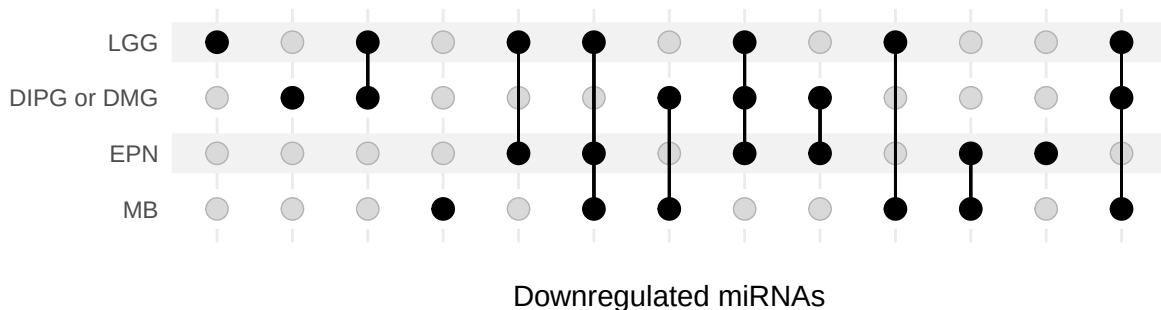
UpSet: Downregulated miRNAs (Tumor vs Healthy Normal)
