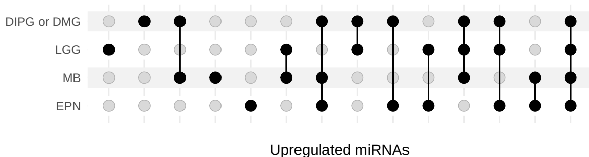
UpSet: Upregulated miRNAs (Tumor vs Healthy Normal)
