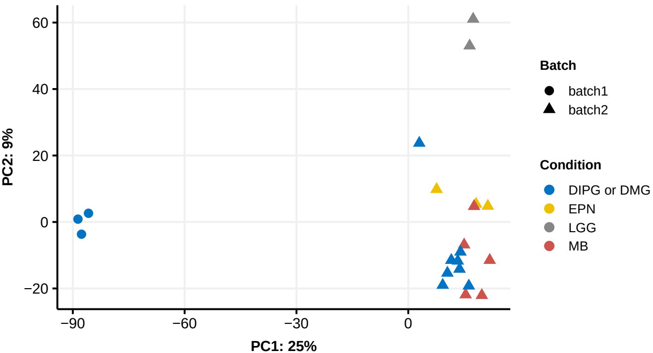
PCA: Tumor Only (Uncorrected)
