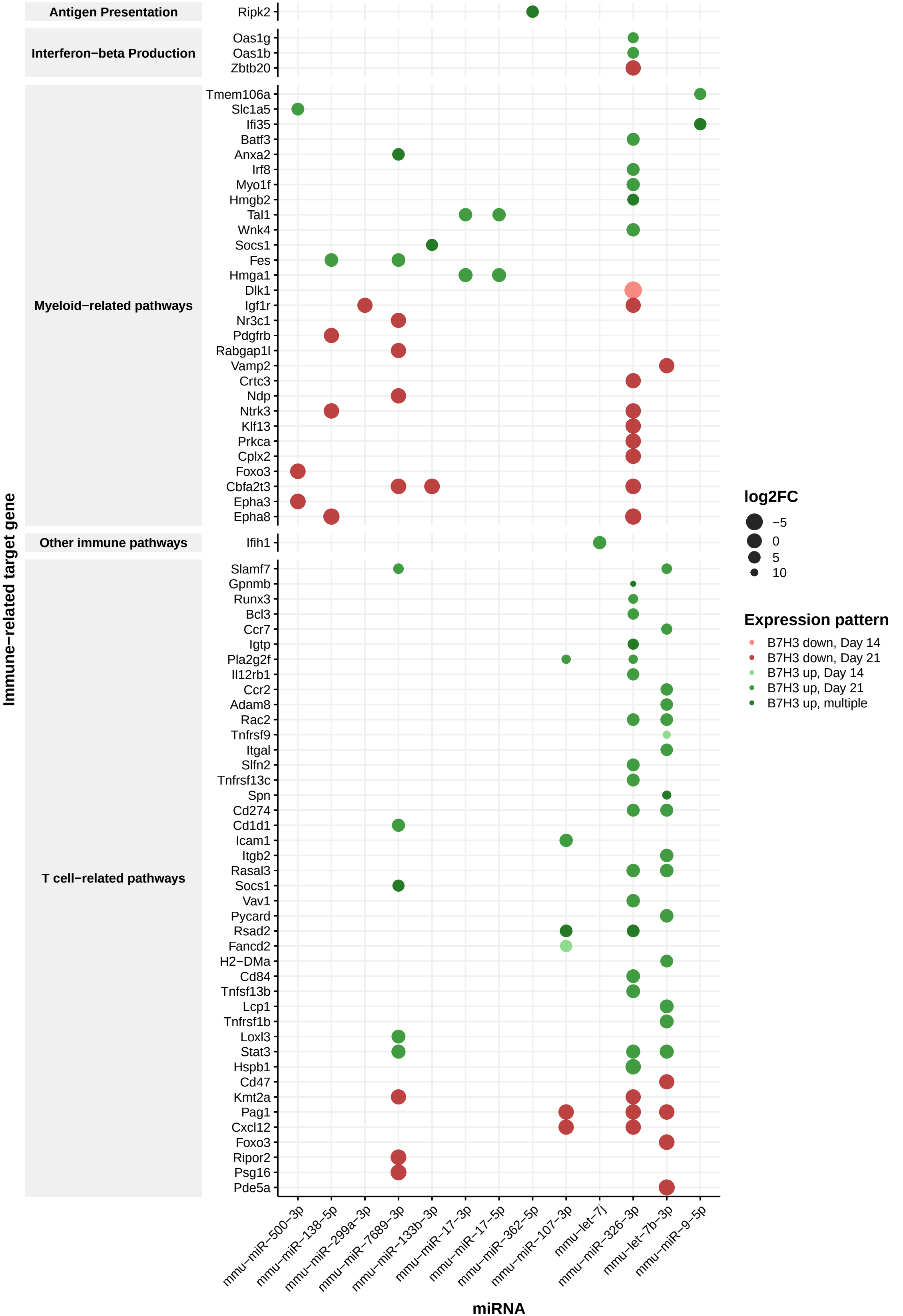
miRNA–Immune Target Interactions (Full – cluster5)
