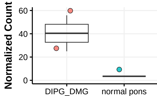
S100A9
