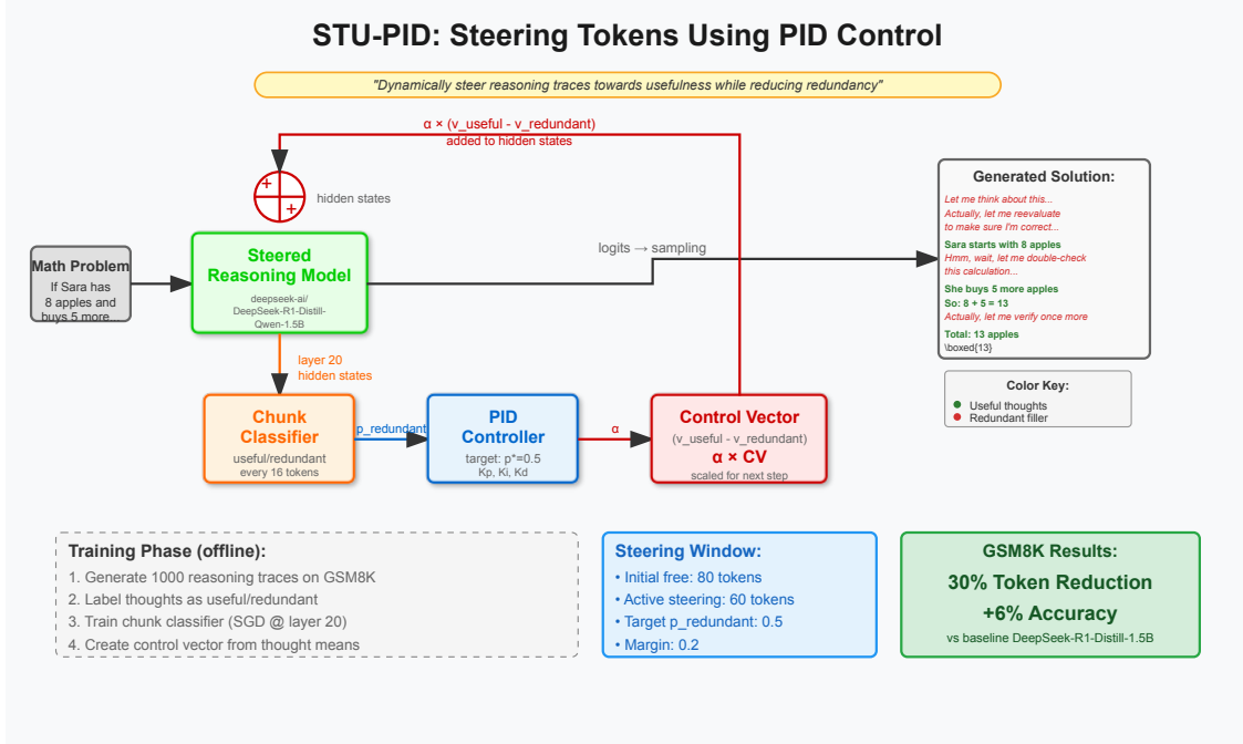
Figure 1: Method overview. The classifier scores each reasoning chunk; the PID controller turns the redundancy error into a steering coefficient \alpha_t applied to the layer- l residual stream.
