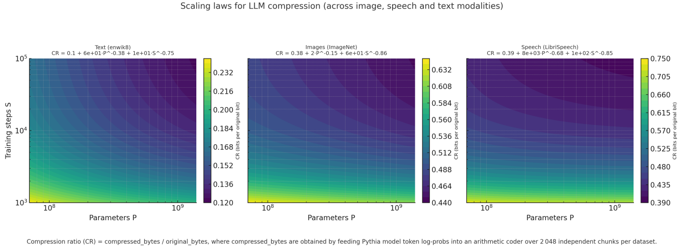
Figure 1: Scaling laws for LLM compression across text, image, and speech modalities. The heatmaps show compression ratio as a function of model parameters (P) and training steps (S). Lower compression ratios (darker colors) indicate better compression performance. Each modality follows the power law \text{CR}(P, S) = a + bP^{-\alpha} + cS^{-\beta} with modality-specific coefficients shown in the equations above each subplot.
