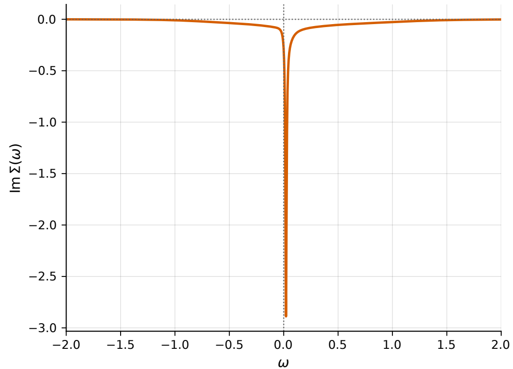
self-energy: overview
