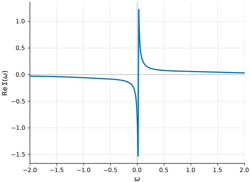
self-energy: overview
