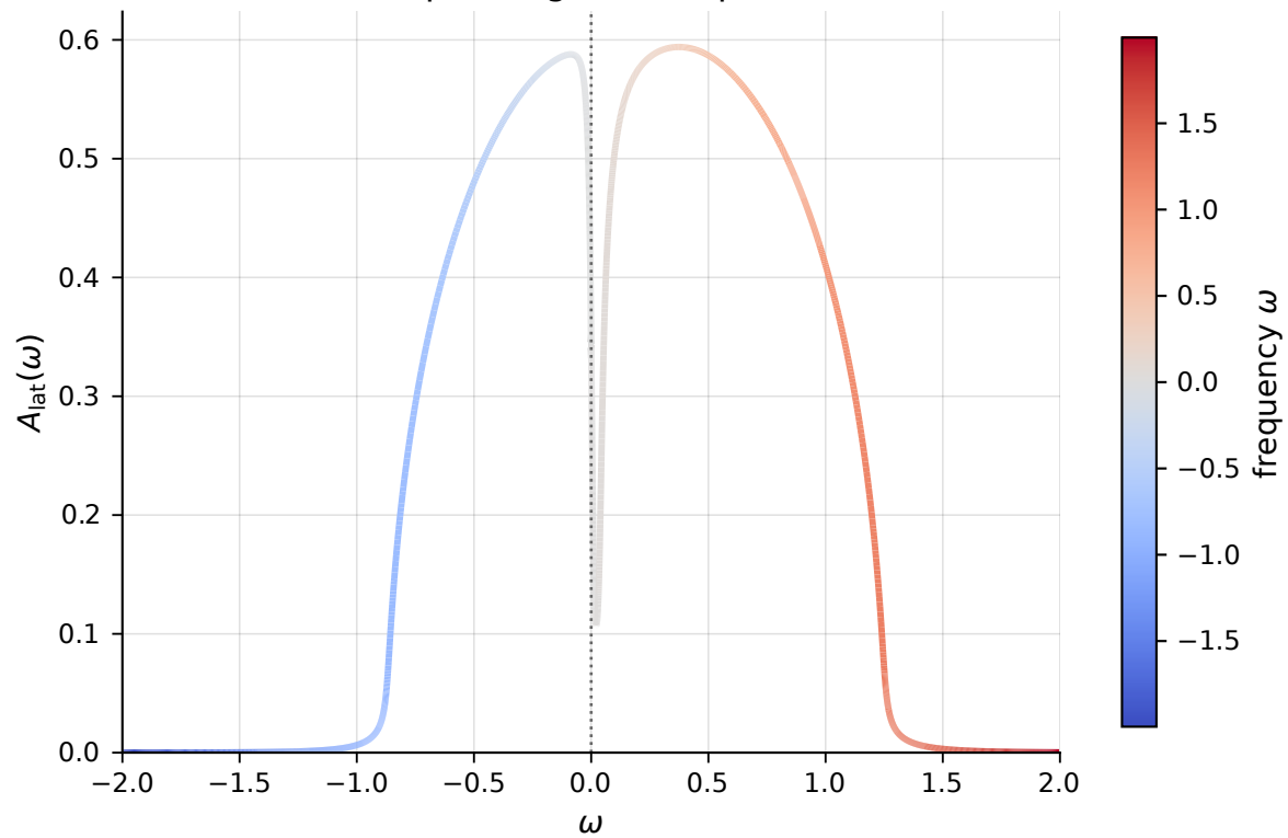
corresponding lattice spectrum
