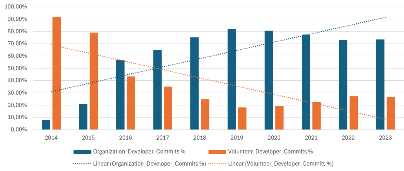
Commits
