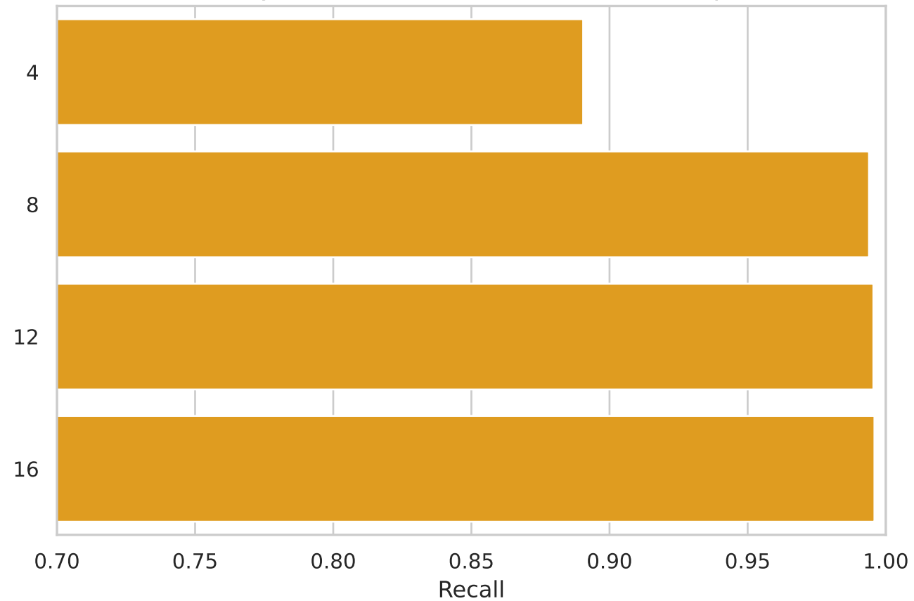
Recall by Camera Count (Fixed at YLO26n-pose)
