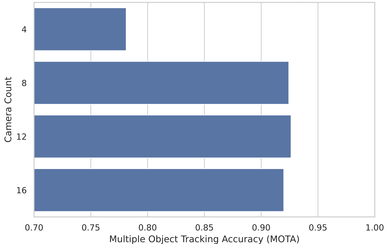
MOTA by Camera Count (Fixed at YLO26n-pose)
