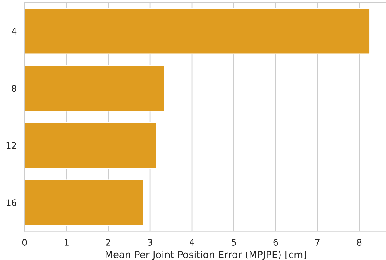
MPJPE by Camera Count (Fixed at YLO26n-pose)
