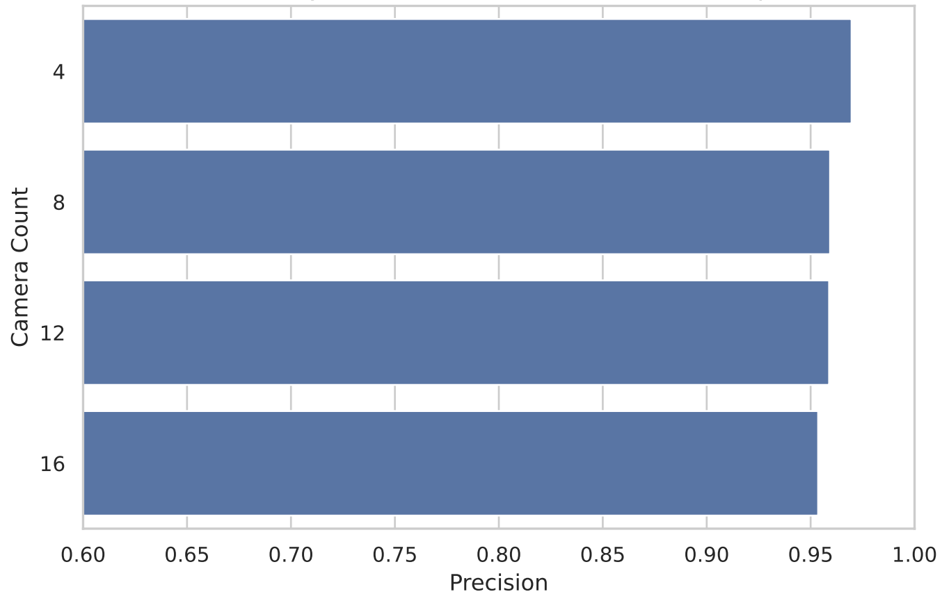
Precision by Camera Count (Fixed at YLO26n-pose)
