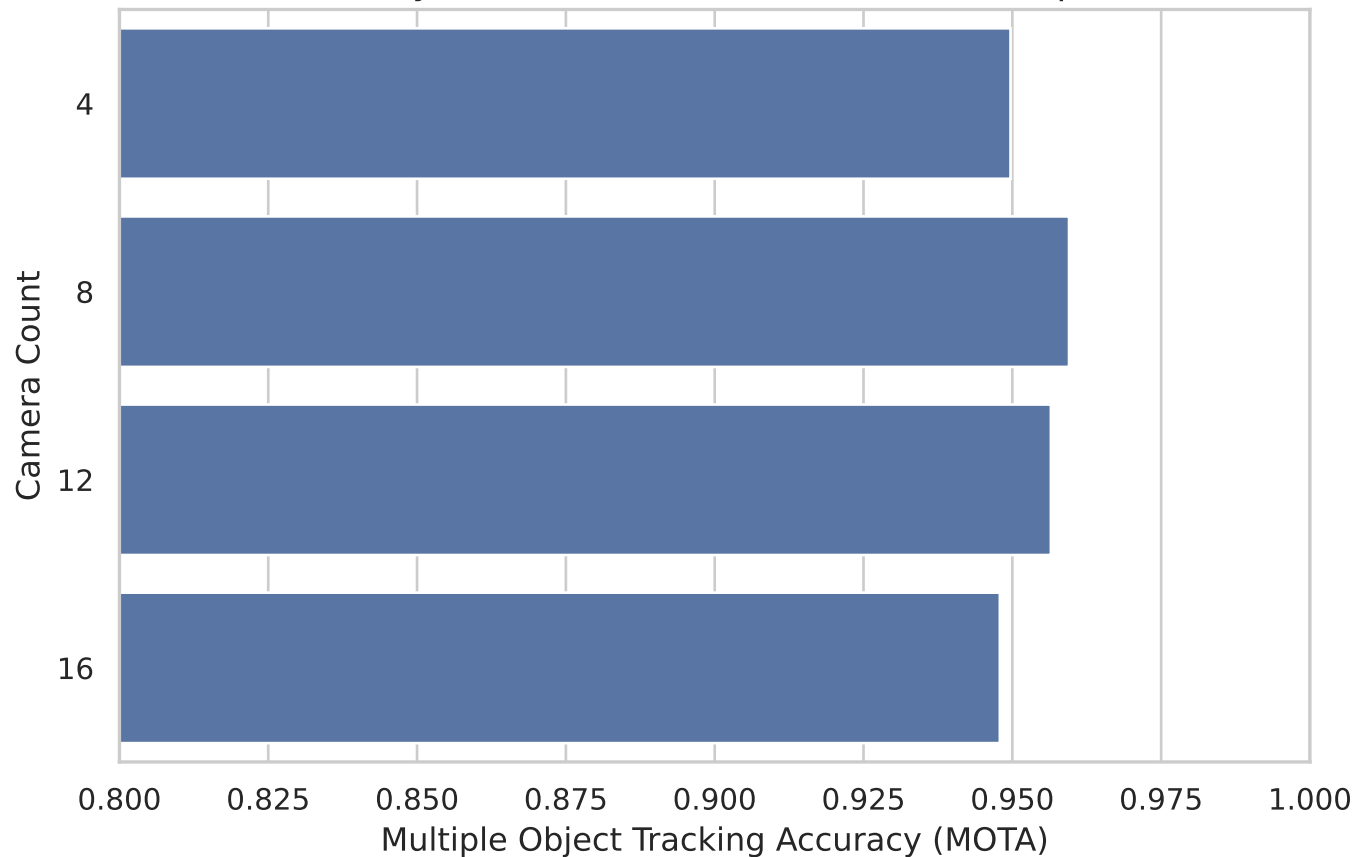
MOTA by Camera Count (Fixed at YLO26n-pose)
