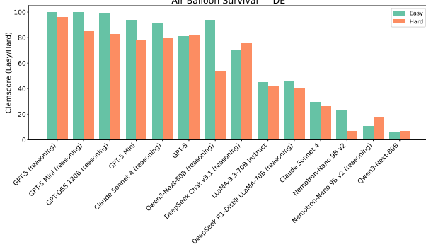
(b) Clem scores on German instances.
