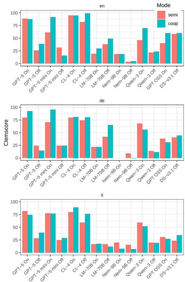
Figure 19: Clemscore for different models separated by language and game mode.
