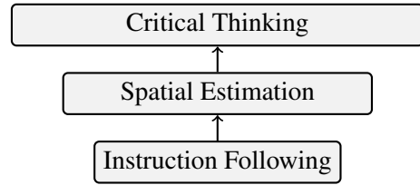
Figure 33: Capability Hierarchical
