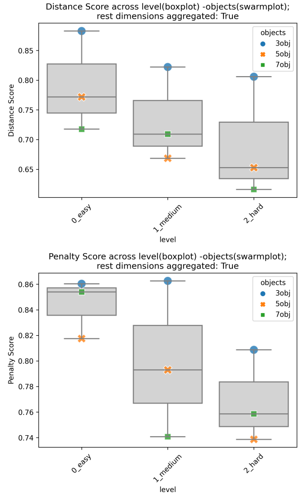
Figure 30: Sub Scores across levels and sub-levels
