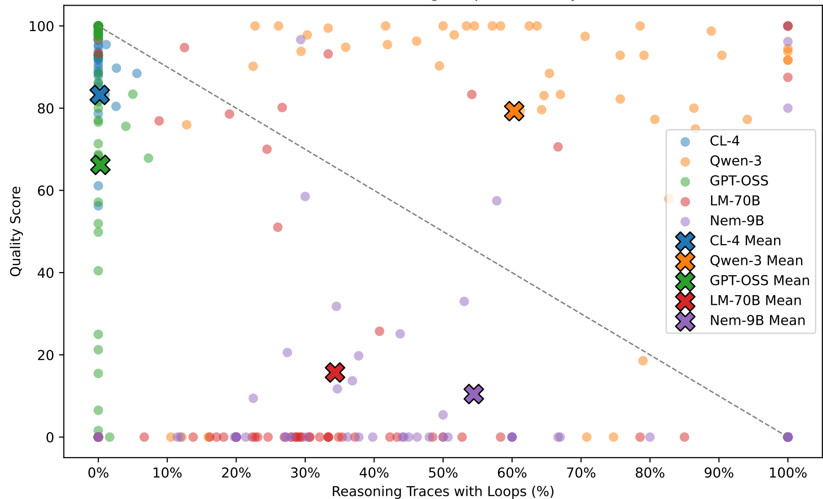
Presence of Reasoning Loops vs Quality Score
