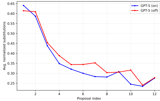
Figure 42: Substitutions over proposals in temporal order for GPT-5. Values are averaged over proposals at each time step in a negotiation across all experiments and languages.
