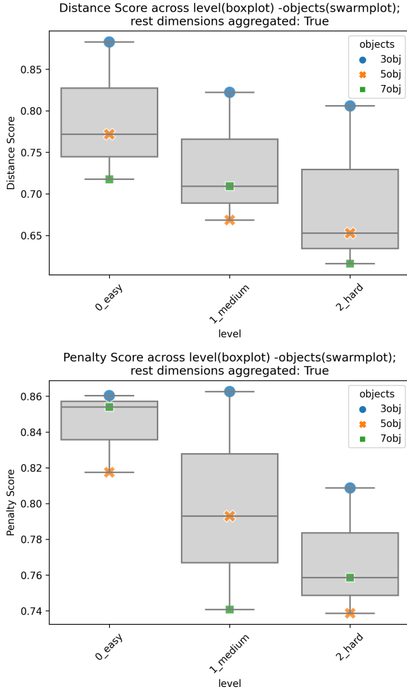
Figure 29: Sub Scores across levels and sub-levels
