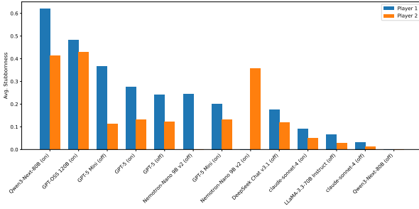
Figure 41: Average per-player per-instance stubbornness for each model across languages on opposing-goals instances.
