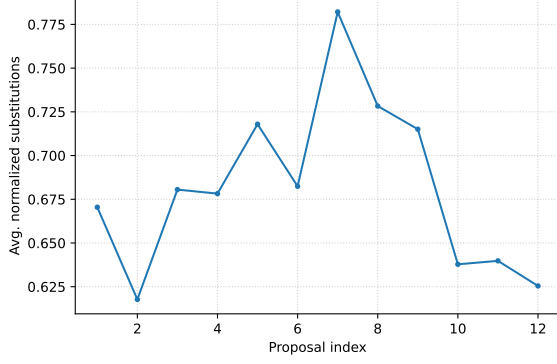
Figure 44: Average normalised substitutions over proposals in temporal order for GPT-OSS 120B.
