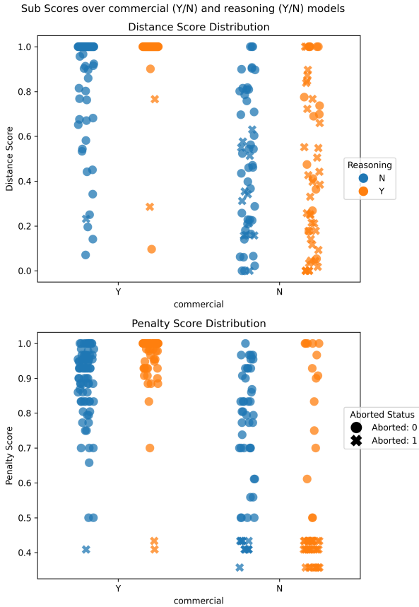
Figure 31: Sub Scores over different model properties
