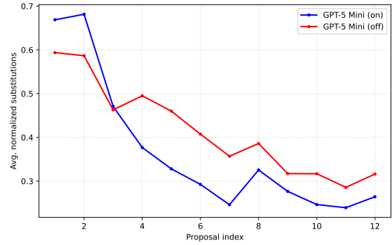
Figure 43: Average normalised substitutions over proposals in temporal order for GPT-5 Mini.
