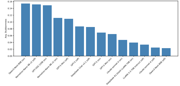
Figure 40: Average per-instance stubbornness per model across languages and experiments.
