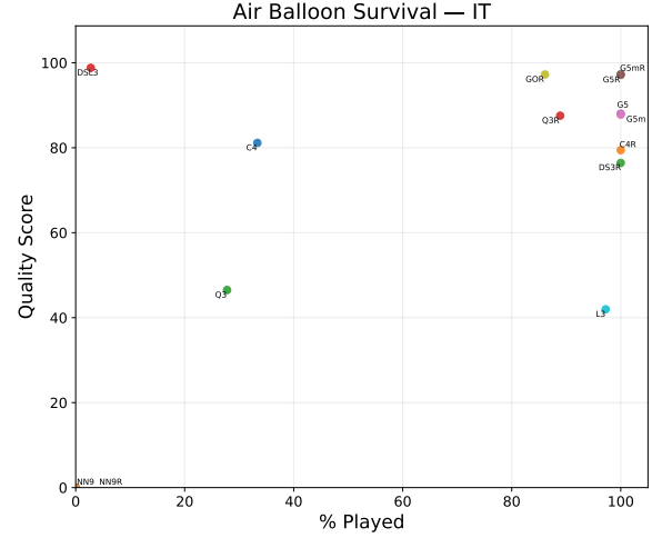
Figure 39: Quality and Played scores on Air Balloon Survival (Italian). Scatters are annotated with acronyms of model names. ‘R’ denotes reasoning model.
