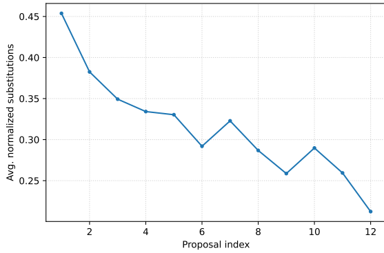
Figure 45: Average normalised substitutions over proposals in temporal order for DeepSeek Chat v3.1.
