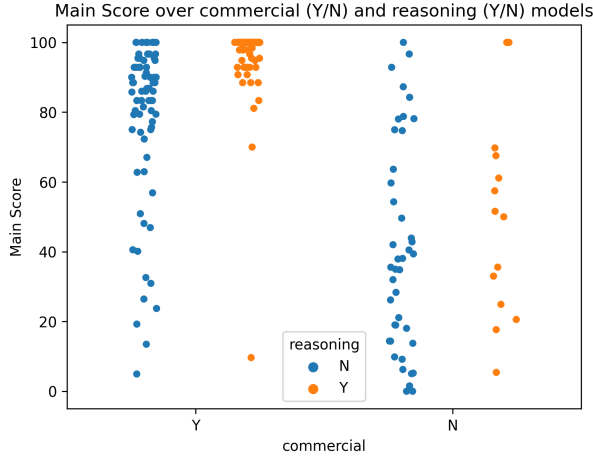
Figure 30: Main Score over different model properties
