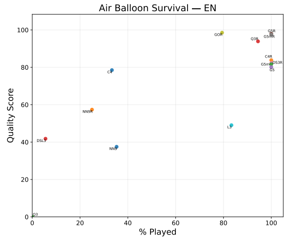
Figure 37: Quality and Played scores on Air Balloon Survival (English). Scatters are annotated with acronyms of model names. ‘R’ denotes reasoning model.
