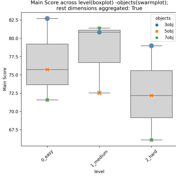
Figure 28: Main Score across levels and sub-levels
