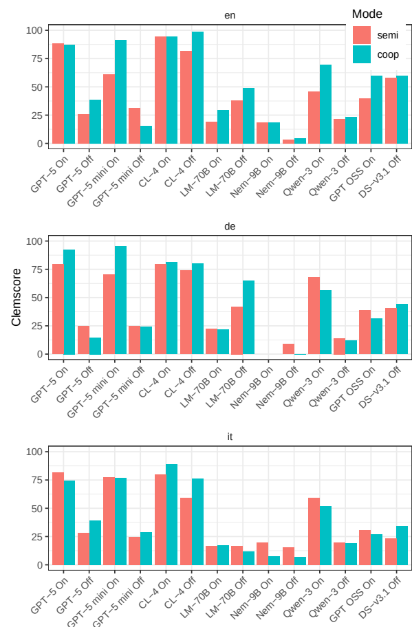
Figure 12: Clemscores for different models seperated by language and game mode.
