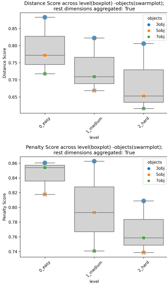
Figure 19: Sub Scores across levels and sub-levels
