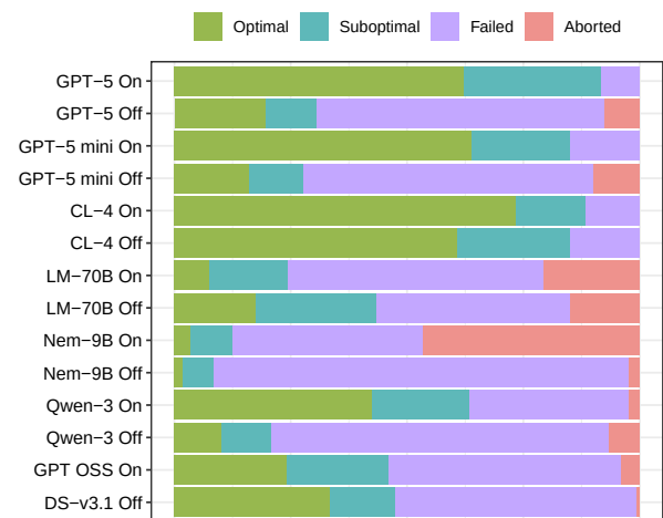
Figure 13: Percentage of games that ended with a specific game outcome during the evaluation of different models. All results for the two game modes and three languages have been averaged together for this plot.
