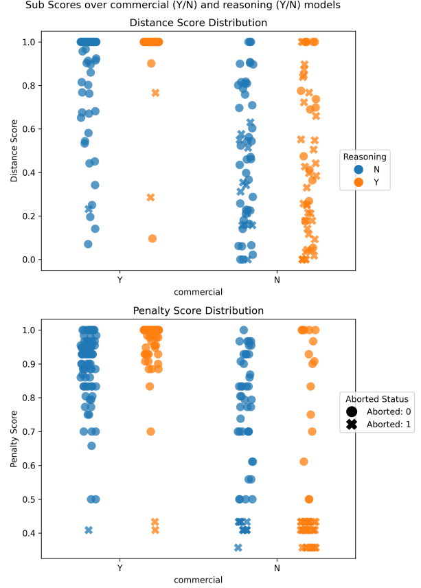
Figure 34: Sub Scores over different model properties
