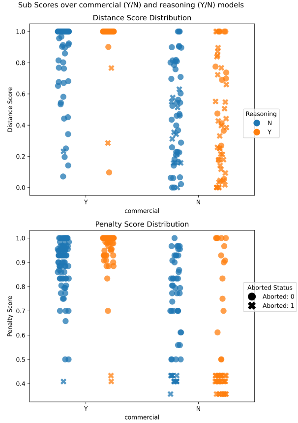
Figure 34: Sub Scores over different model properties
