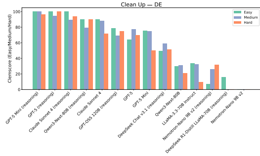
(b) Results for each experiment for German.
