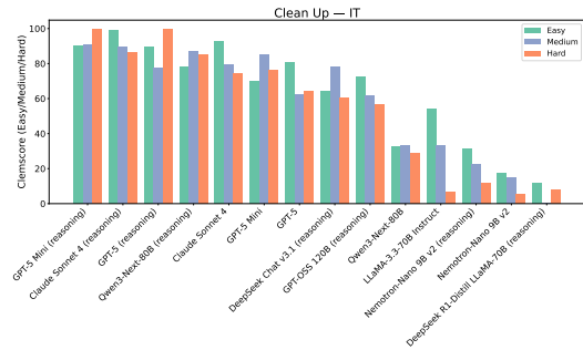
(c) Results for each experiment for Italian.
