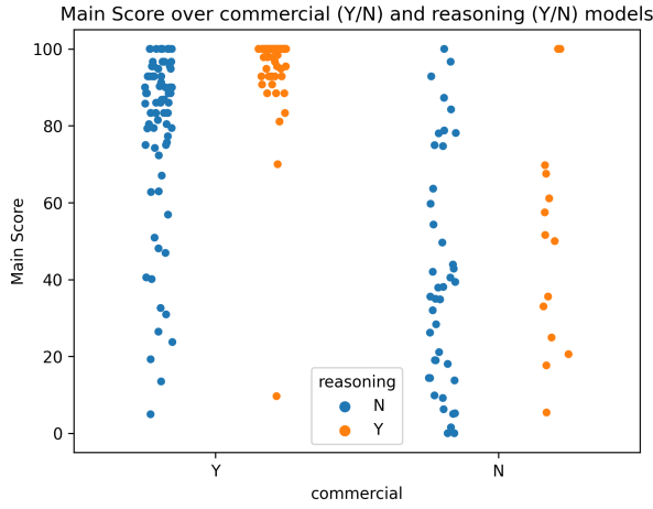
Figure 33: Main Score over different model properties
