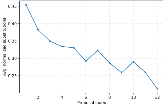
Figure 48: Average normalised substitutions over proposals in temporal order for DeepSeek Chat v3.1.
