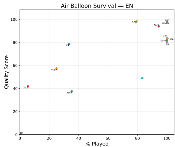
Figure 40: Quality and Played scores on Air Balloon Survival (English). Scatters are annotated with acronyms of model names. ‘R’ denotes reasoning model.
