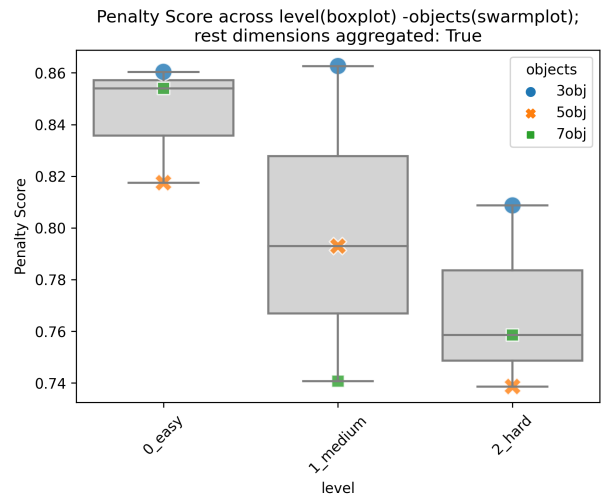
Figure 32: Sub Scores across levels and sub-levels
