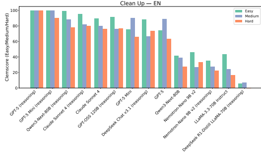
(a) Results for each experiment for English.
