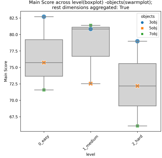
Figure 31: Main Score across levels and sub-levels
