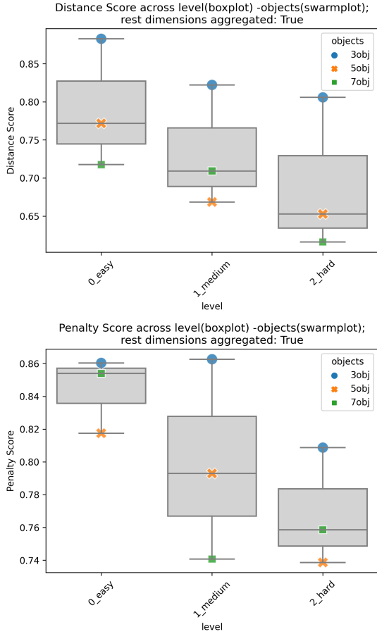
Figure 32: Sub Scores across levels and sub-levels
