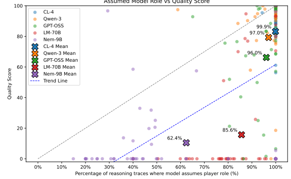
(d) Percentage of reasoning traces where the model assumes a player role, as opposed to an assistant/helper role, plotted vs. a quality score. 95.2% of data points are below the main diagonal, meaning a model rarely reaches a quality score higher than the percentage of reasoning traces where it assumes a player role.
