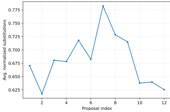
Figure 47: Average normalised substitutions over proposals in temporal order for GPT-OSS 120B.
