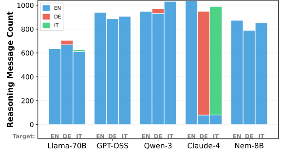
Figure 6: Language distribution in reasoning tokens
