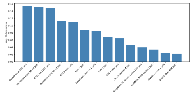
Figure 43: Average per-instance stubbornness per model across languages and experiments.
