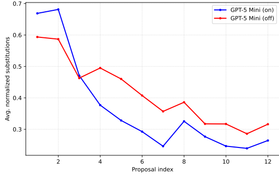
Figure 46: Average normalised substitutions over proposals in temporal order for GPT-5 Mini.
