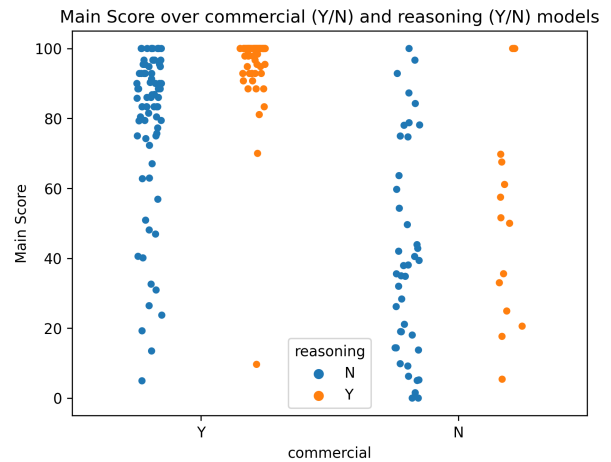
Figure 16: Main Score over different model properties
