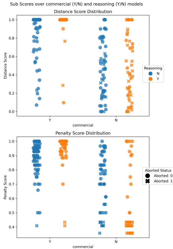
Figure 17: Sub Scores over different model properties
