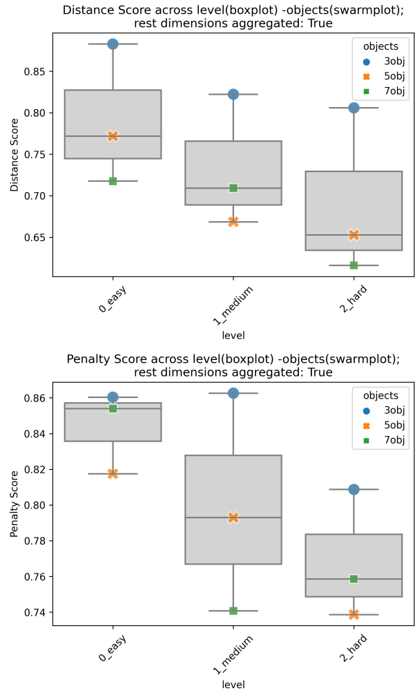
Figure 15: Sub Scores across levels and sub-levels
