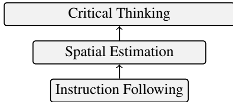
Figure 18: Capability Hierarchical
