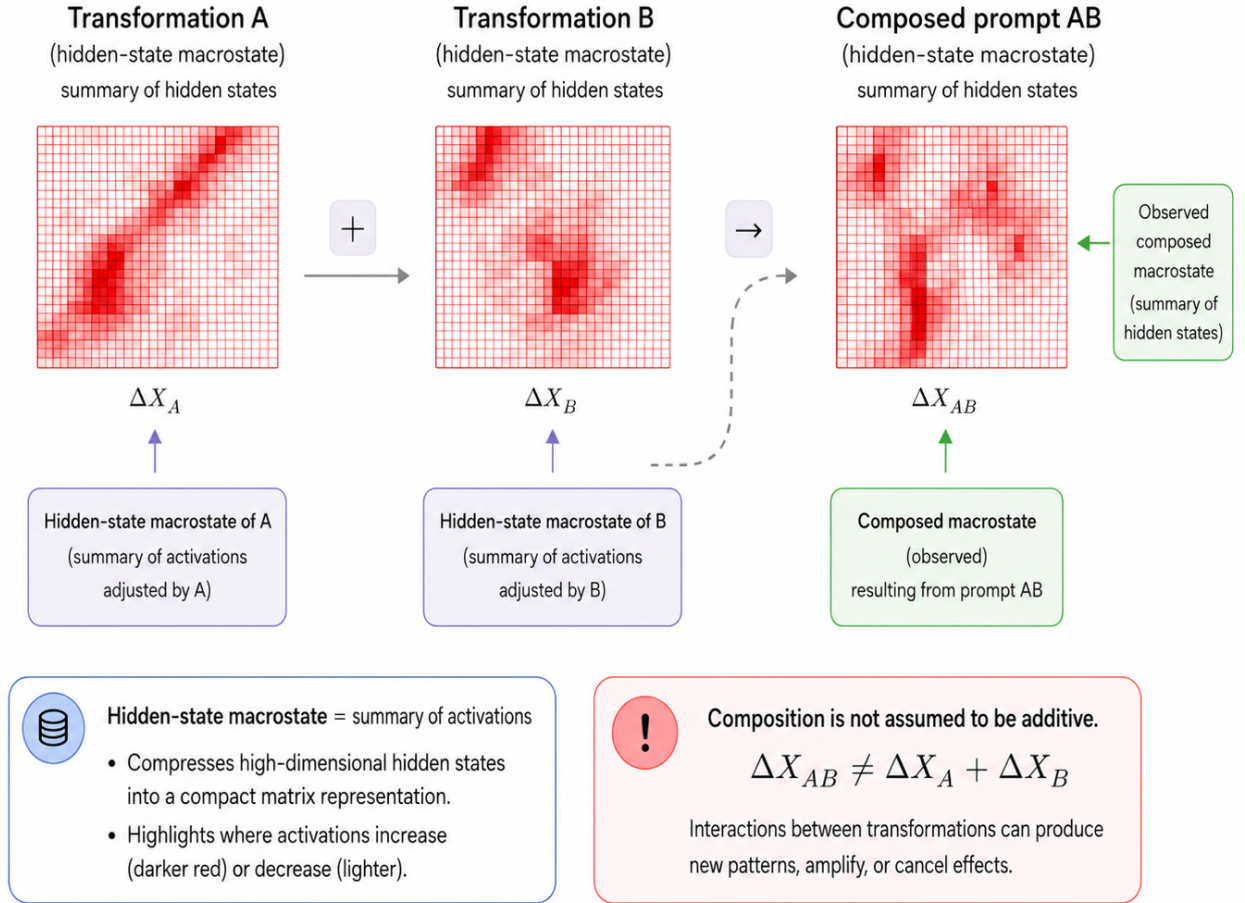
Figure 2: Conceptual view of hidden-state macrostates. Each prompt transformation induces a compact matrix-valued summary of hidden-state activations. The composed prompt AB induces its own observed macrostate \Delta X_{AB} , which is not assumed to coincide with the additive superposition \Delta X_A + \Delta X_B . This figure is schematic and is intended to provide intuition for macrostate composition.
