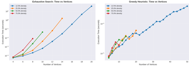
Fig. 1. Execution time comparison showing exponential growth for exhaustive search (left) versus polynomial scaling for greedy heuristic (right) across all four required edge densities. The log-scale visualization clearly demonstrates the dramatic performance difference between complexity classes.
