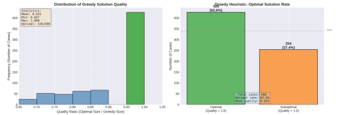
Fig. 2. Distribution of greedy solution quality showing that 62.6% of cases achieve optimal solutions (quality ratio = 1.0) with the remaining 37.4% achieving near-optimal solutions. The mean quality ratio of 0.925 demonstrates excellent practical performance.
