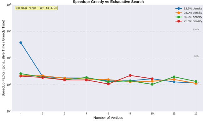
Fig. 3. Speedup analysis comparing greedy heuristic against exhaustive search. The speedup ranges from 10 \times to 379 \times , demonstrating consistent order-of-magnitude performance improvements across all densities and vertex counts.
